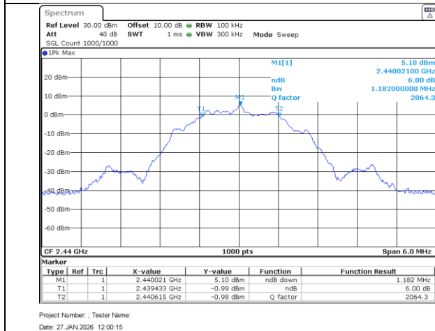
Mid Ch_2440MHz_2MBit_Occupied Bandwidth_ - 6dB
