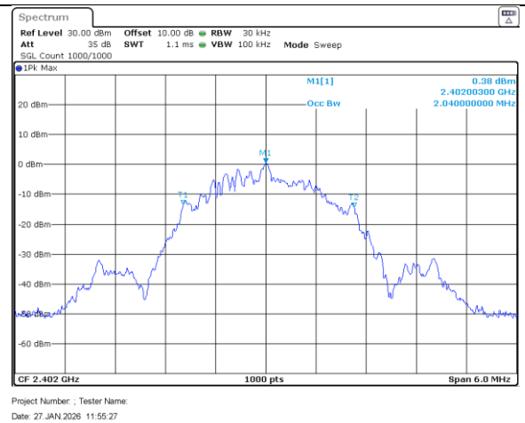
Low Ch_2402MHz_2MBit_Occupied Bandwidth_99 percent
