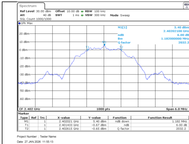
Low Ch_2402MHz_2MBit_Occupied Bandwidth_ - 6dB
