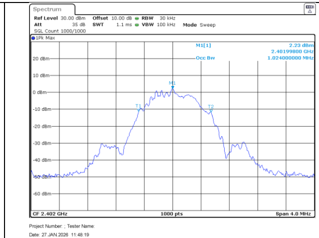
Low Ch_2402MHz_1MBit_Occupied Bandwidth_99 percent
