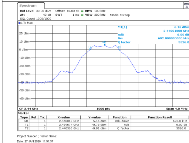
Mid Ch_2440MHz_1MBit_Occupied Bandwidth_-6dB
