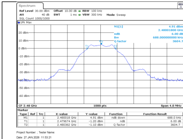
High Ch_2480MHz_1MBit_Occupied Bandwidth_ - 6dB
