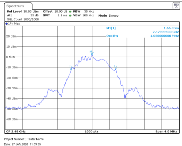
High Ch_2480MHz_1MBit_Occupied Bandwidth_99 percent
