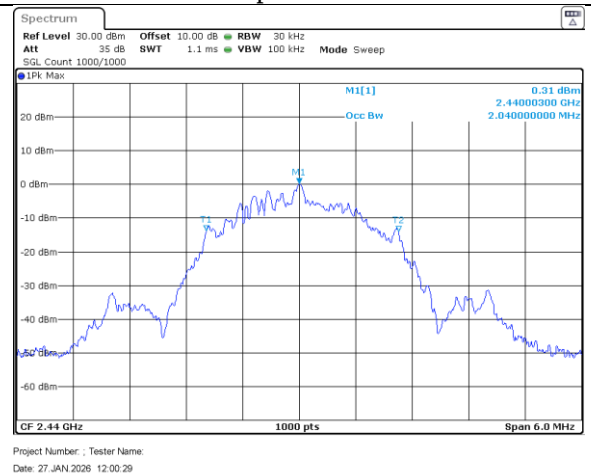
Mid Ch_2440MHz_2MBit_Occupied Bandwidth_99 percent
