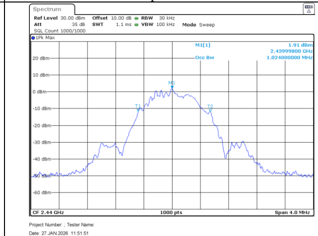
Mid Ch_2440MHz_1MBit_Occupied Bandwidth_99 percent
