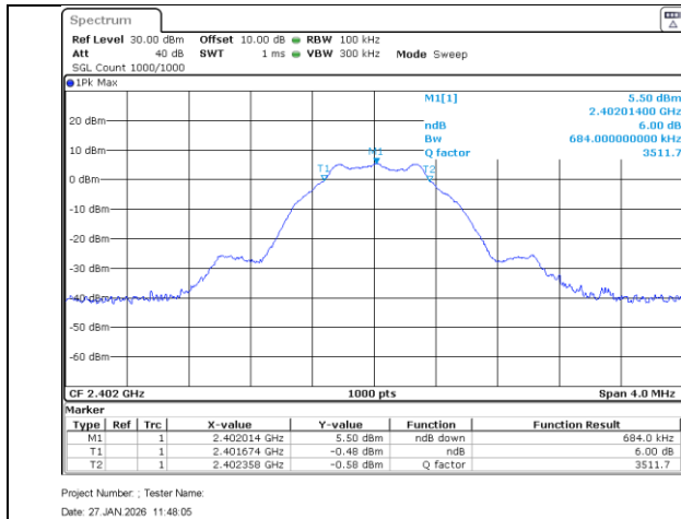
Low Ch_2402MHz_1MBit_Occupied Bandwidth_-6dB
