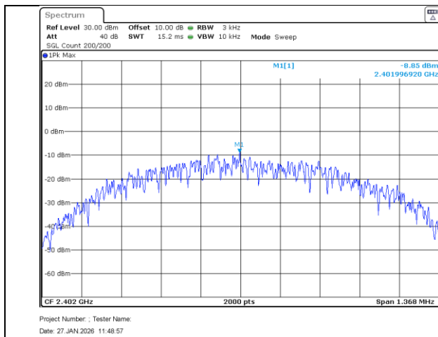
BLE_Low Ch_2402MHz_1MBit_Spectral Density
