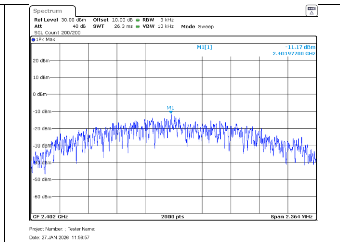
BLE_Low Ch_2402MHz_2MBit_Spectral Density
