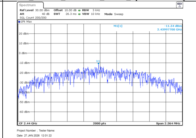
BLE_Mid Ch_2440MHz_2MBit_Spectral Density
