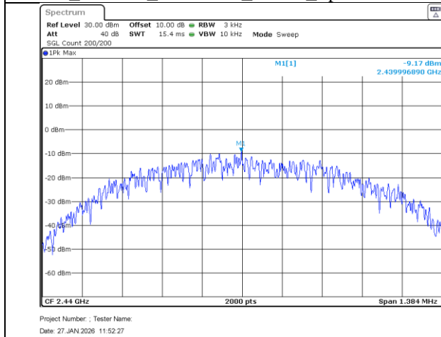
BLE_Mid Ch_2440MHz_1MBit_Spectral Density
