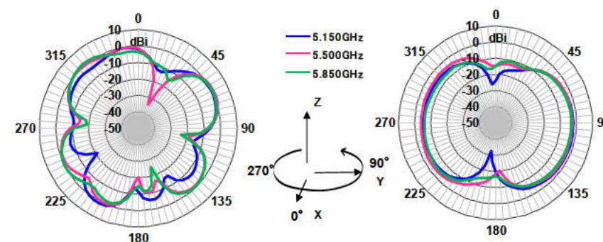
Horizontal Polarization
