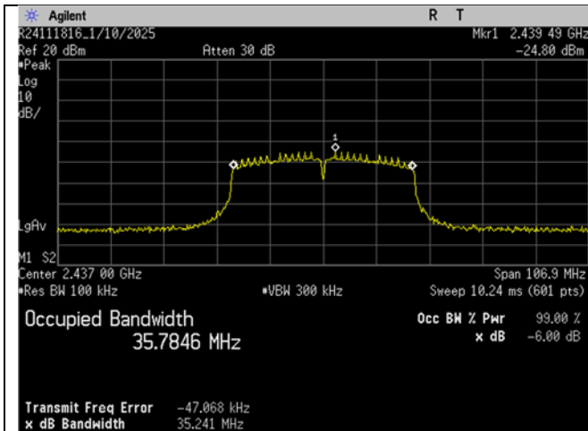
WiFi_Mid Ch_2437MHz_40MHz BW_n- mode_Occupied Bandwidth_-6dB
