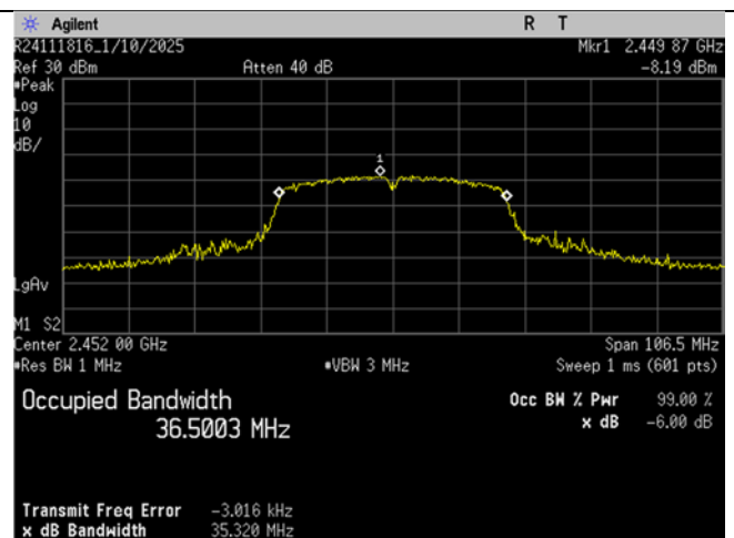
WIFI_High Ch_2452MHz_40MHz BW_n-mode_Occupied Bandwidth_99 percent
