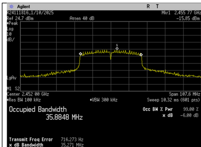
WIFI_High Ch_2452MHz_40MHz BW_n-mode_Occupied Bandwidth_-6dB
