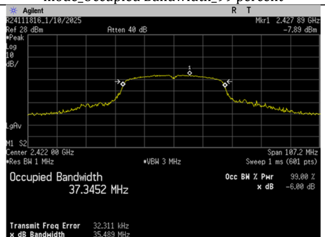
WIFI_Low Ch_2422MHz_40MHz BW_n-mode_Occupied Bandwidth_99 percent
