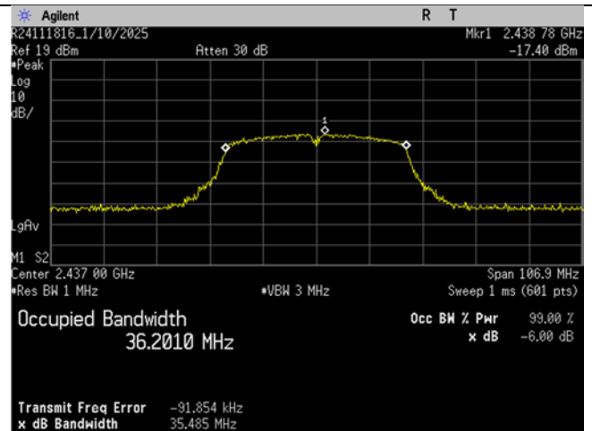
WiFi_Mid Ch_2437MHz_40MHz BW_n- mode_Occupied Bandwidth_99 percent
