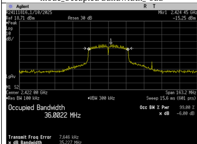
WIFI_Low Ch_2422MHz_40MHz BW_n-mode_Occupied Bandwidth_-6dB
