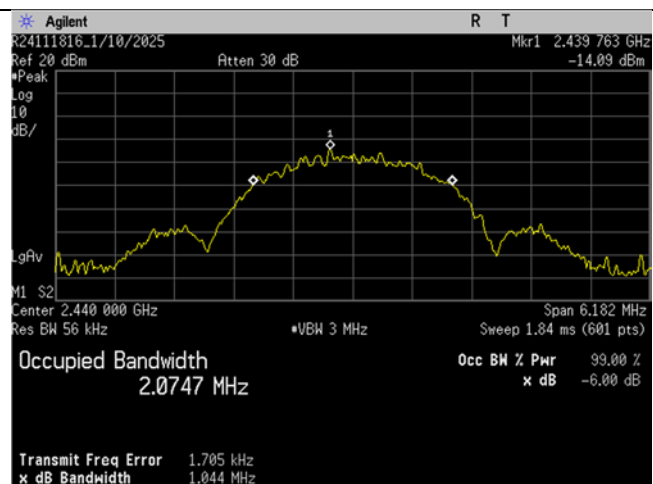
BLE_Mid Ch_2440MHz_2MBit_Occupied Bandwidth_99 percent
