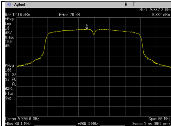
U-NII-2C_5590MHz_Mid Ch_118_40MHz BW_n/ac -mode_Spectral Density
