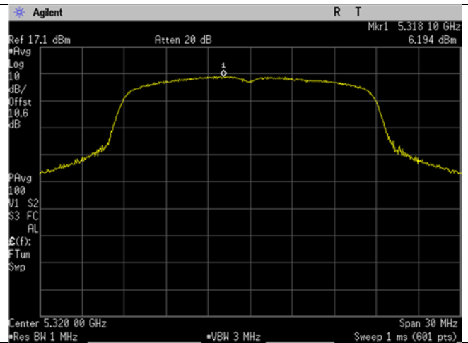
U-NII-2A_5320MHz_High Ch_64_20MHz BW_n/ac-mode_Spectral Density
