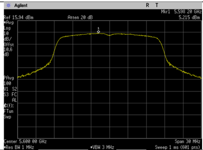
U-NII-2C_5600MHz_Mid Ch_120_20MHz BW_a- mode_Spectral Density
