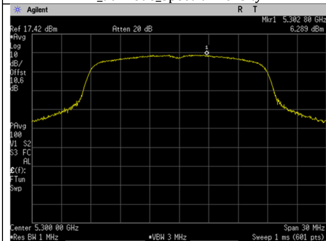
U-NII-2A_5300MHz_high_Mid Ch_60_20MHz BW_n/ac -mode_Spectral Density
