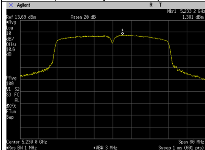
U-NII-1_5230MHz_high_Mid Ch_46_40MHz BW_n/ac -mode_Spectral Density
