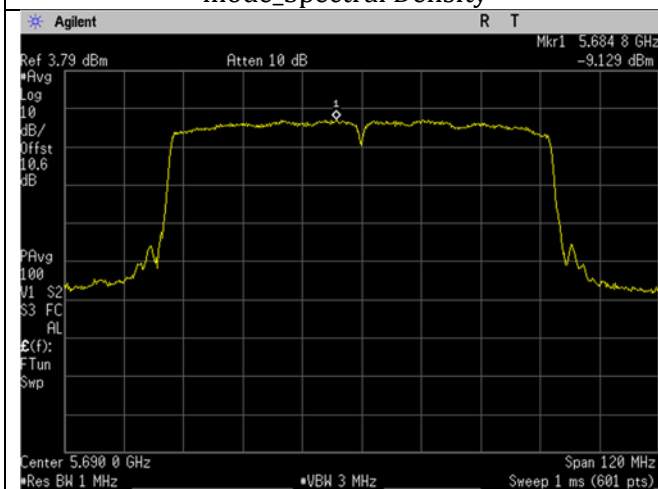
U-NII-2C_5690MHz_High Ch_138_80MHz BW_ac- mode_Spectral Density
