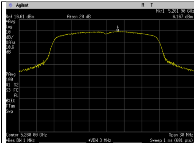
U-NII-2A_5260MHz_low_mid Ch_52_20MHz BW_n/ac -mode_Spectral Density
