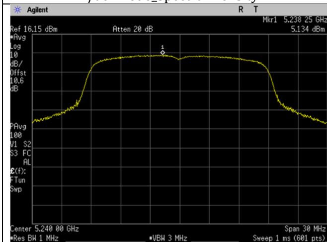
U-NII-1_5240MHz_high_mid Ch_48_20MHz BW_n/ac -mode_Spectral Density
