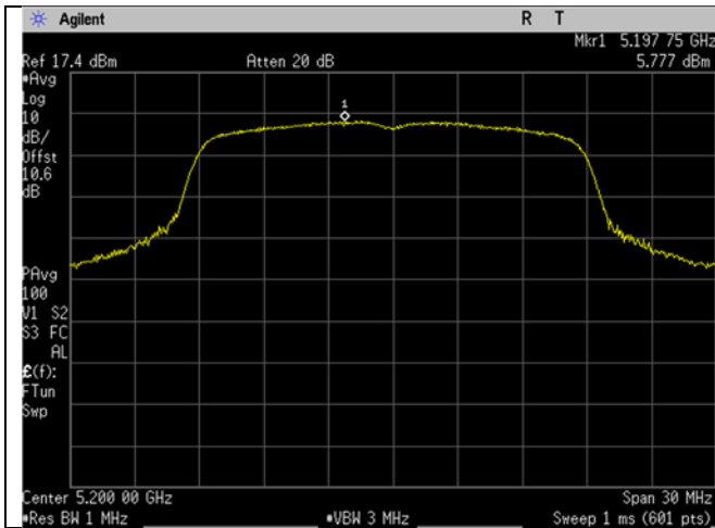
U-NII-1_5200MHz_low_Mid Ch_40_20MHz BW_n/ac -mode_Spectral Density
