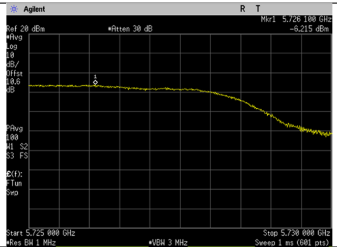
n/ac40mode 5710 MHz straddle right
