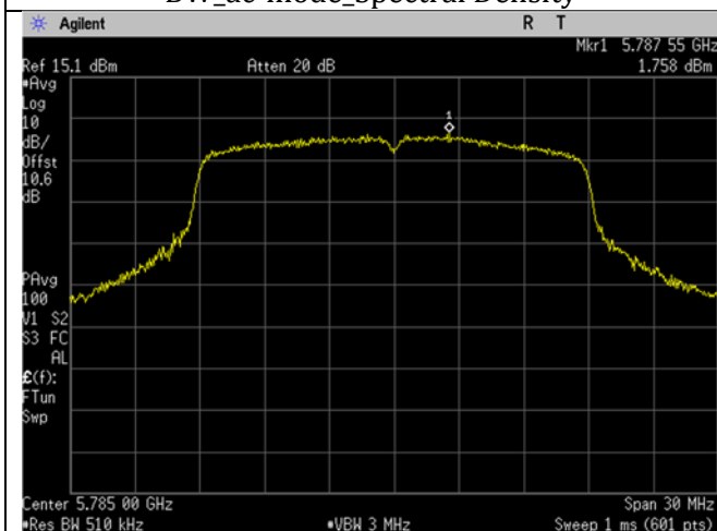
U-NII-3_5785MHz_Mid Ch_157_20MHz BW_n/ac - mode_Spectral Density
