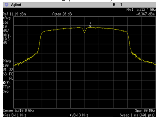
U-NII-2A_5310MHz_High Ch_62_40MHz BW_n/ac -mode_Spectral Density
