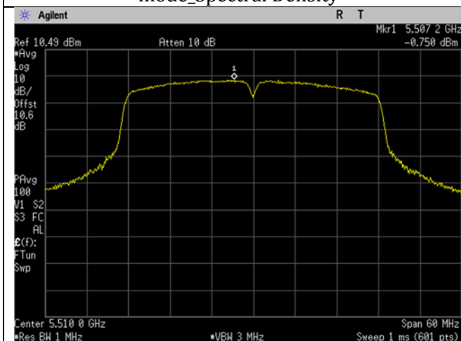
U-NII-2C_5510MHz_Low Ch_102_40MHz BW_n/ac-mode_Spectral Density
