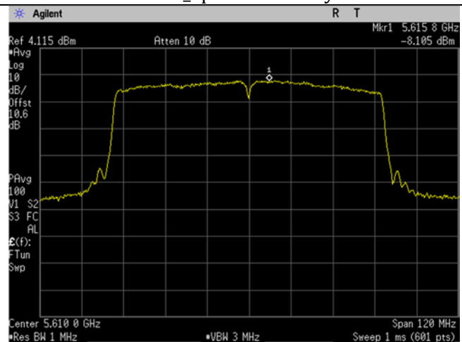
U-NII-2C_5610MHz_Mid Ch_122_80MHz BW_ac- mode_Spectral Density
