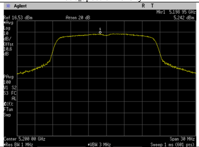
U-NII-1_5200MHz_low_Mid Ch_40_20MHz BW_a-mode_Spectral Density
