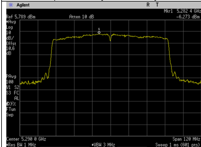
U-NII-2A_5290MHz_High_Mid Ch_58_80MHz BW_ac-mode_Spectral Density
