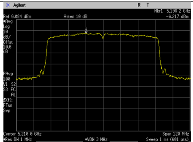
U-NII-1_5210MHz_Low Mid Ch_42_80MHz BW_ac-mode_Spectral Density
