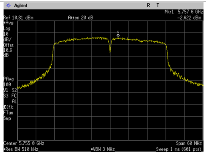
U-NII-3_5755MHz_Low Ch_151_40MHz BW_n/ac - mode_Spectral Density
