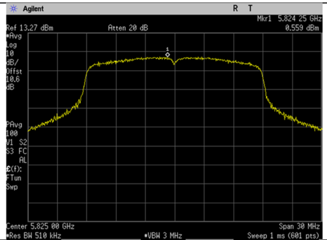
U-NII-3_5825MHz_High Ch_165_20MHz BW_n/ac -mode_Spectral Density
