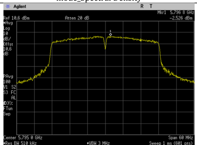
U-NII-3_5795MHz_High_Mid Ch_159_40MHz BW_n/ac - mode_Spectral Density
