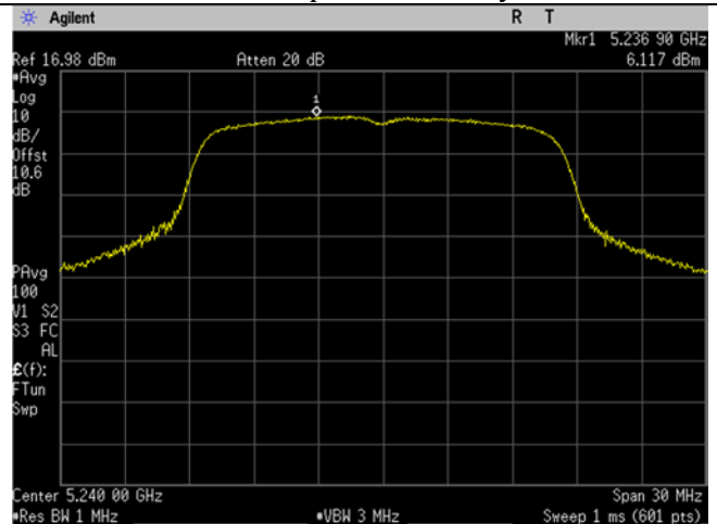
U-NII-1_5240MHz_high_mid Ch_48_20MHz BW_a-mode_Spectral Density
