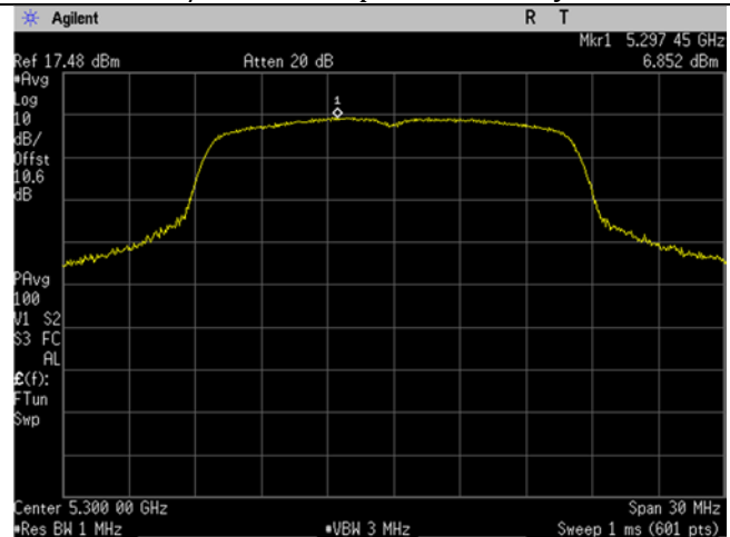
U-NII-2A_5300MHz_high_Mid Ch_60_20MHz BW_a-mode_Spectral Density
