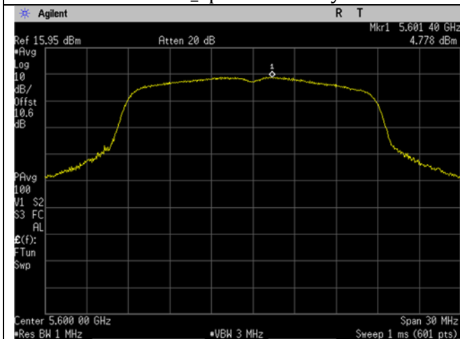
U-NII-2C_5600MHz_Mid Ch_120_20MHz BW_n/ac -mode_Spectral Density
