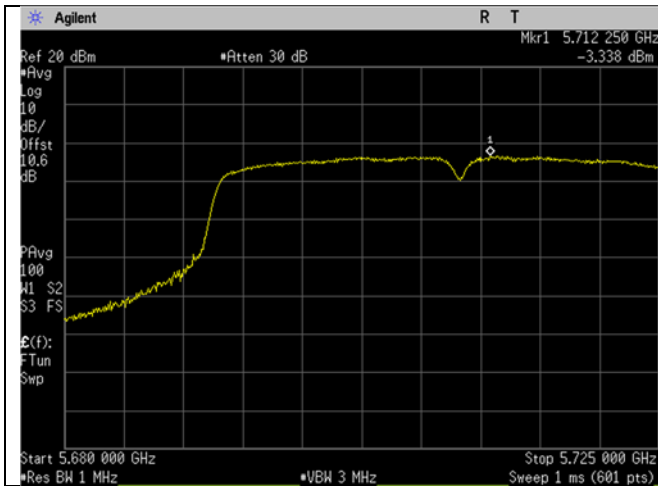
n/ac40mode 5710 MHz straddle left
