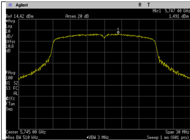
U-NII-3_5745MHz_Low Ch_149_20MHz BW_n/ac - mode_Spectral Density
