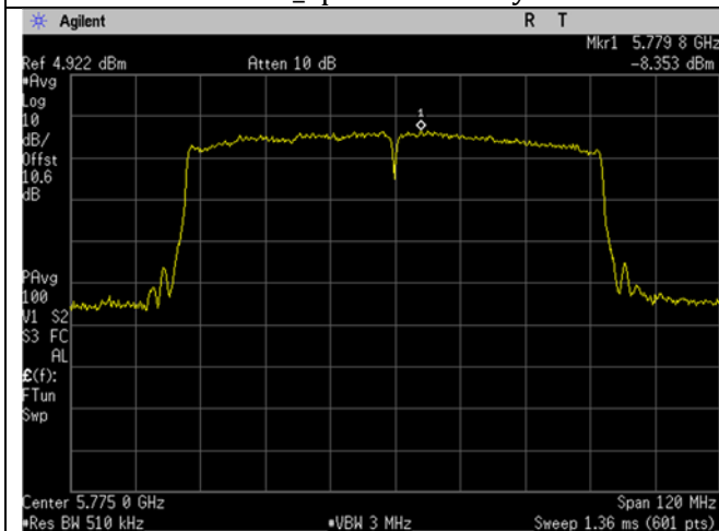
U-NII-3_5775MHz_High_Mid Ch_155_80MHz BW_ac-mode_Spectral Density
