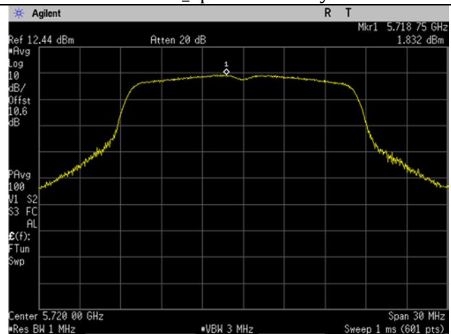
U-NII-2C_5720MHz_High Ch_144_20MHz BW_a-mode_Spectral Density
