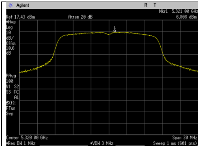
U-NII-2A_5320MHz_High Ch_64_20MHz BW_a-mode_Spectral Density
