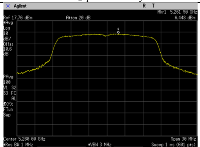
U-NII-2A_5260MHz_low_mid Ch_52_20MHz BW_a-mode_Spectral Density
