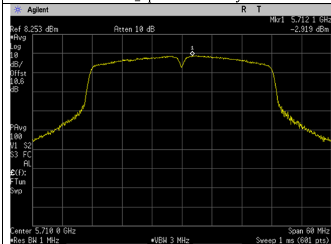
U-NII-2C_5710MHz_High Ch_142_40MHz BW_n/ac-mode_Spectral Density
