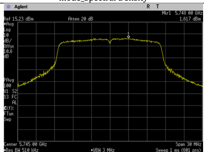
U-NII-3_5745MHz_Low Ch_149_20MHz BW_a-mode_Spectral Density
