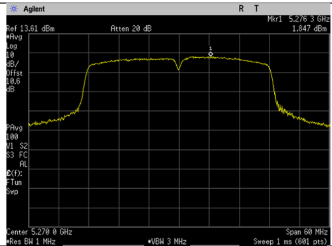
U-NII-2A_5270MHz_low_Mid Ch_54_40MHz BW_n/ac -mode_Spectral Density
