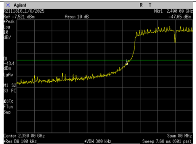
WIFI_Low Ch_2422MHz_40MHz BW_n-mode_- 30dBc_Lower Band Edge
