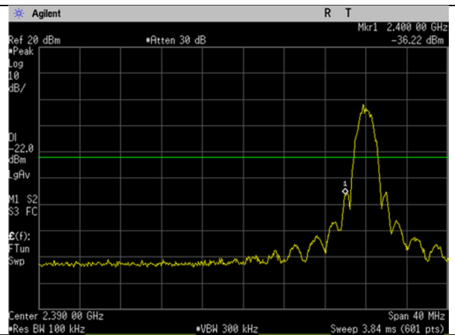
BLE_Low CH_2402MHz_2MHz BW_Mbit_20dBc Lower Band Edge
