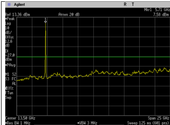
U-NII-2C_5710MHz_High Ch_142_40MHz BW_n/ac-mode_-27dBm_1-26GHz
