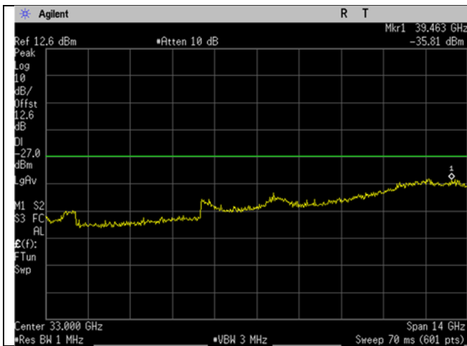
U-NII-3_5755MHz_Low Ch_151_40MHz BW_n/ac- mode_-27dBm_26-40GHz_Peak
