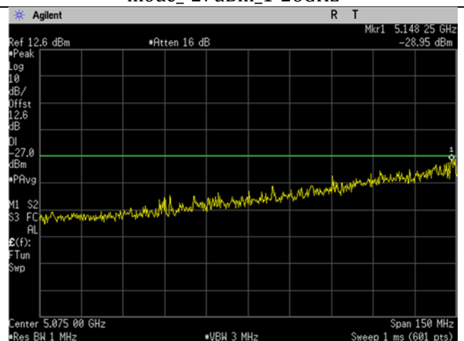
U-NII-1_5210MHz_Low Mid Ch_42_80MHz BW_ac- mode_-27dBm_Lower Band Edge
