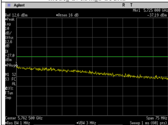
U-NII-2C_5700MHz_High Ch_140_20MHz BW_a-mode_-27dBm_Upper Band Edge
