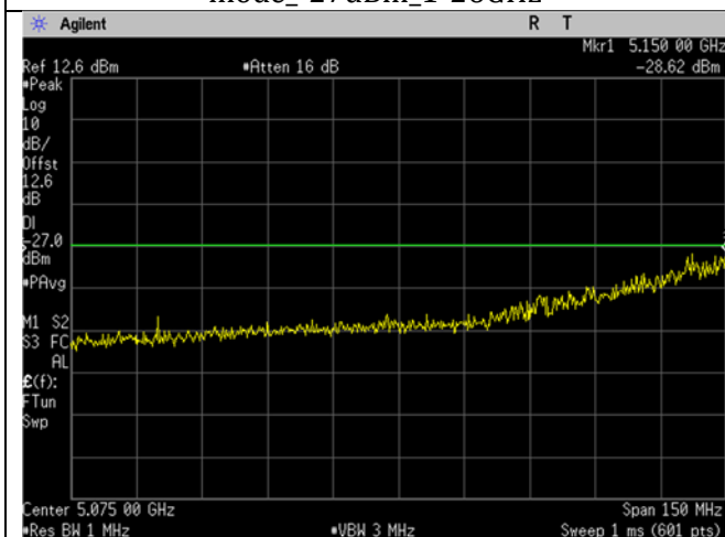
U-NII-1_5190MHz_Low Ch_38_40MHz BW_n/ac-mode_-27dBm_Lower Band Edge
