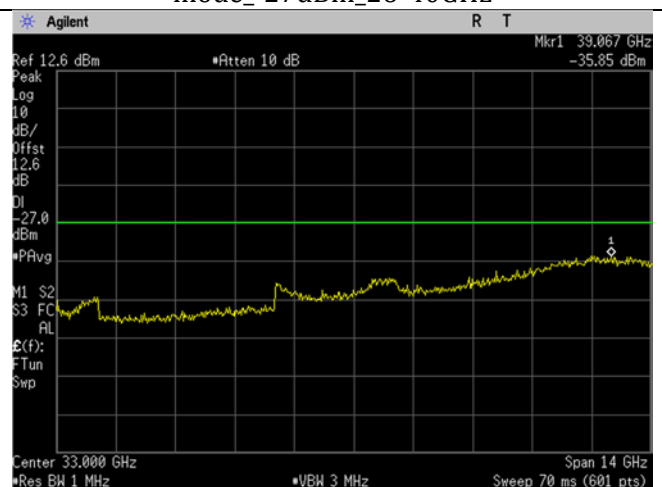
U-NII-1_5240MHz_high_mid Ch_48_20MHz BW_n/ac-mode_-27dBm_26-40GHz
