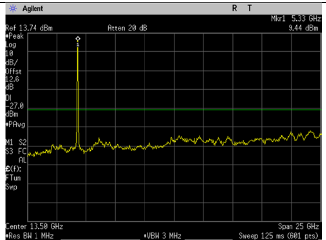
U-NII-2A_5310MHz_High Ch_62_40MHz BW_n/ac- mode_-27dBm_1-26GHz
