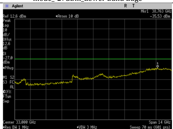
U-NII-2C_5590MHz_Mid Ch_118_40MHz BW_n/ac-mode_-27dBm_26-40GHz
