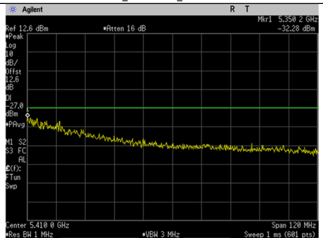
U-NII-2A_5310MHz_High Ch_62_40MHz BW_n/ac- mode_-27dBm_Upper Band Edge
