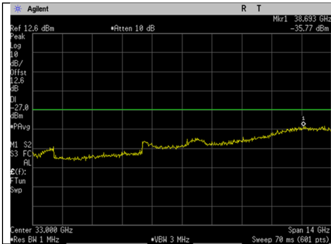
U-NII-2A_5300MHz_high_Mid Ch_60_20MHz BW_n/ac-mode_-27dBm_26-40GHz
