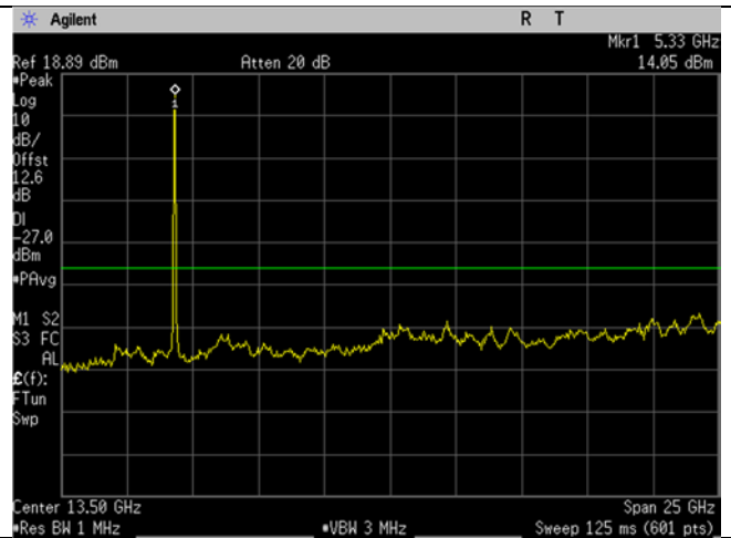
U-NII-2A_5320MHz_High Ch_64_20MHz BW_n/ac-mode_-27dBm_1-26GHz
