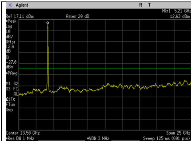
U-NII-1_5230MHz_high_Mid Ch_46_40MHz BW_n/ac-mode_-27dBm_1-26GHz
