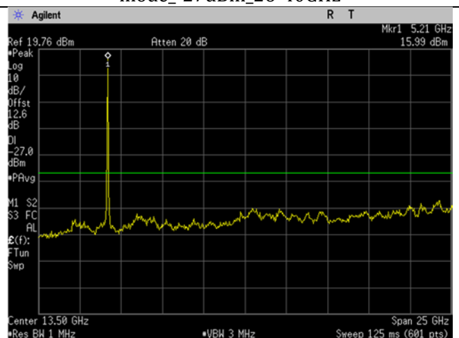
U-NII-1_5200MHz_low_Mid Ch_40_20MHz BW_a-mode_-27dBm_1-26GHz
