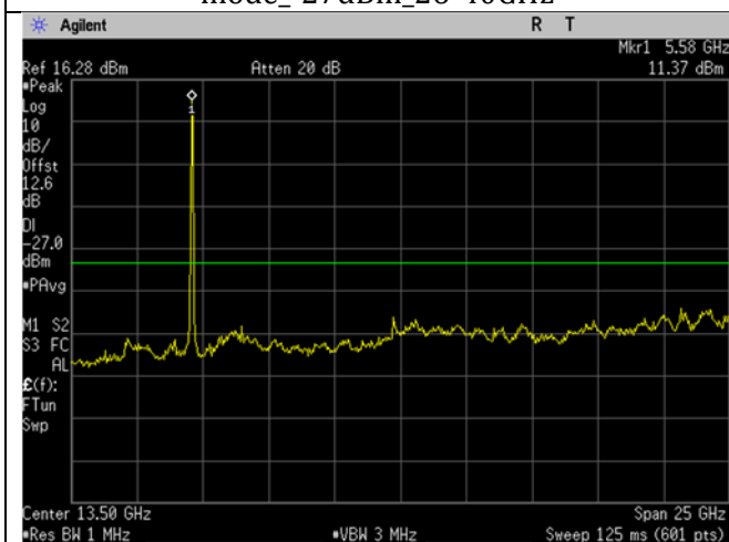
U-NII-2C_5590MHz_Mid Ch_118_40MHz BW_n/ac-mode_-27dBm_1-26GHz
