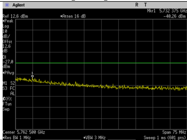
U-NII-2C_5670MHz_High Ch_134_40MHz BW_n/ac-mode_-27dBm_Upper Band Edge
