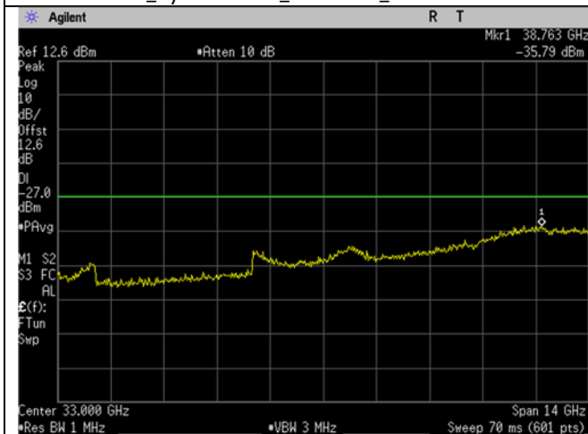
U-NII-2A_5310MHz_High Ch_62_40MHz BW_n/ac- mode_-27dBm_26-40GHz
