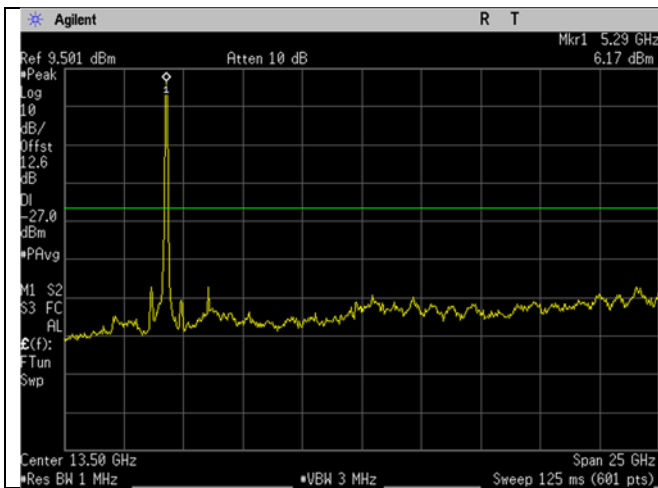
U-NII-2A_5290MHz_High_Mid Ch_58_80MHz BW_ac-mode_-27dBm_1-26GHz
