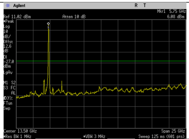
U-NII-3_5775MHz_High_Mid Ch_155_80MHz BW_ac-mode_-27dBm_1-26GHz
