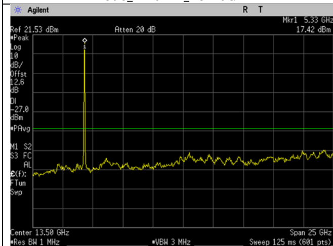
U-NII-2A_5320MHz_High Ch_64_20MHz BW_a- mode_-27dBm_1-26GHz
