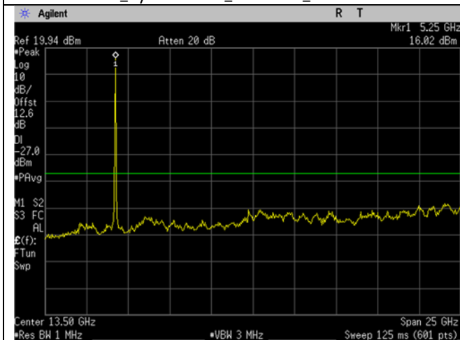
U-NII-1_5240MHz_high_mid Ch_48_20MHz BW_a- mode_-27dBm_1-26GHz
