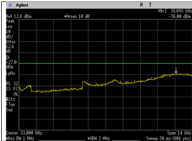
U-NII-3_5785MHz_Mid Ch_157_20MHz BW_n/ac-mode_-27dBm_26-40GHz_Peak
