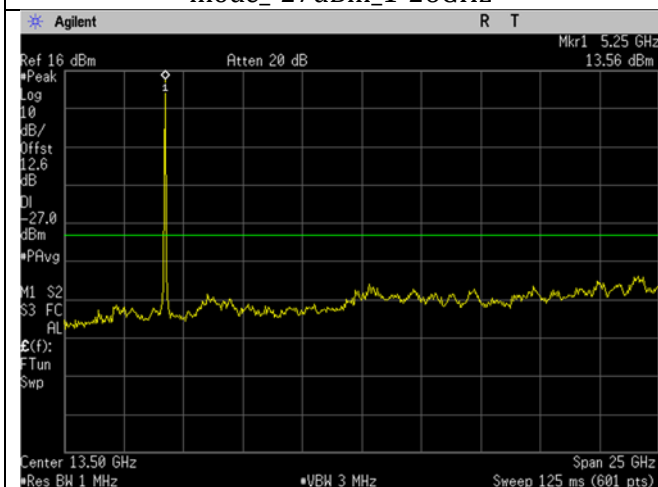
U-NII-1_5240MHz_high_mid Ch_48_20MHz BW_n/ac-mode_-27dBm_1-26GHz
