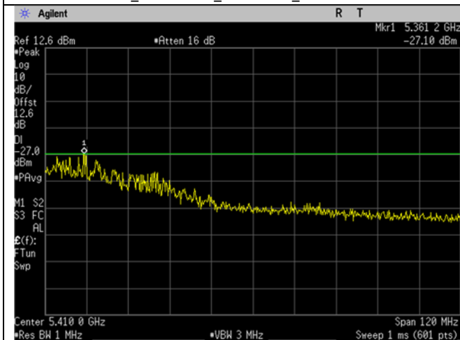
U-NII-2A_5290MHz_High_Mid Ch_58_80MHz BW_ac-mode_-27dBm_Upper Band Edge
