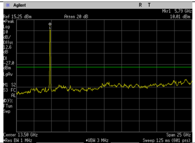
U-NII-3_5795MHz_High_Mid Ch_159_40MHz BW_n/ac-mode_-27dBm_1-26GHz
