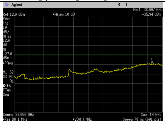
U-NII-1_5240MHz_high_mid Ch_48_20MHz BW_a- mode_-27dBm_26-40GHz
