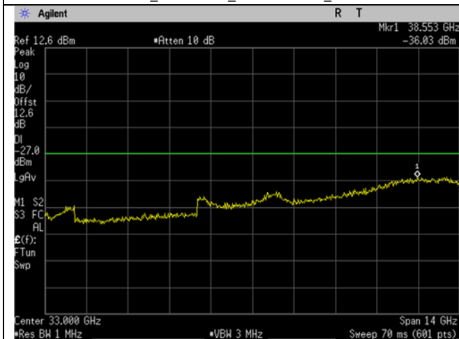
U-NII-3_5775MHz_High_Mid Ch_155_80MHz BW_ac-mode_-27dBm_26-40GHz_Peak
