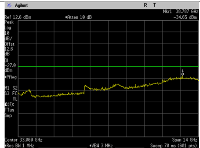
U-NII-2C_5710MHz_High Ch_142_40MHz BW_n/ac-mode_-27dBm_26-40GHz
