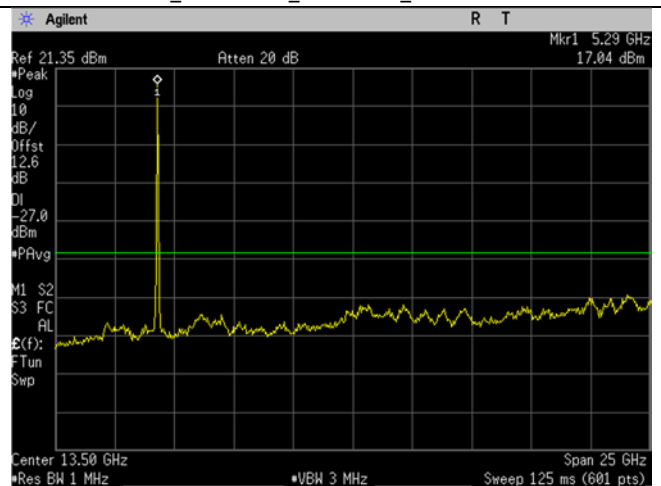
U-NII-2A_5300MHz_high_Mid Ch_60_20MHz BW_a- mode_-27dBm_1-26GHz
