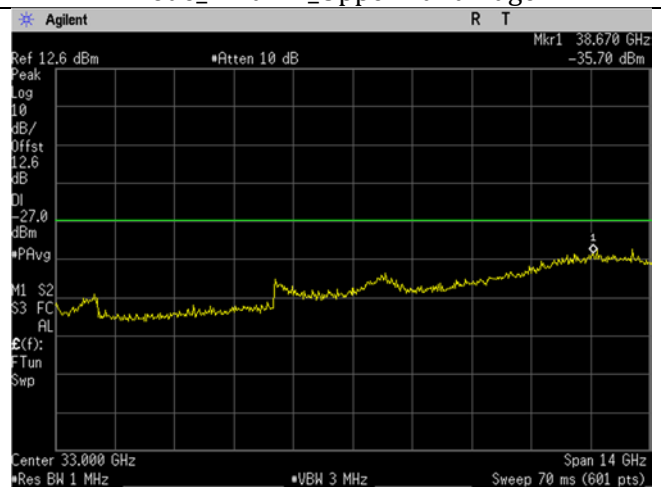
U-NII-2A_5320MHz_High Ch_64_20MHz BW_a- mode_-27dBm_26-40GHz
