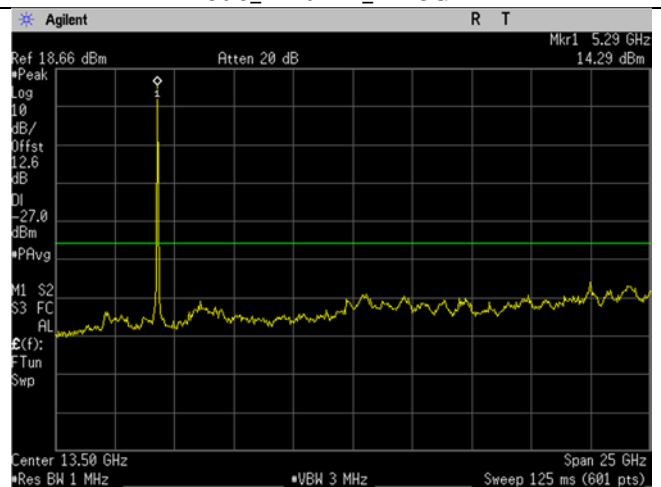
U-NII-2A_5300MHz_high_Mid Ch_60_20MHz BW_n/ac-mode_-27dBm_1-26GHz
