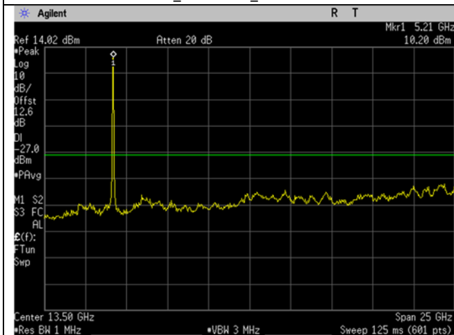
U-NII-1_5190MHz_Low Ch_38_40MHz BW_n/ac-mode_-27dBm_1-26GHz
