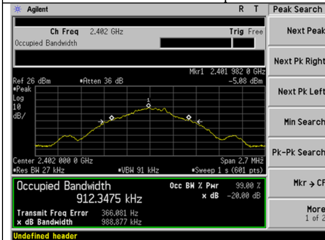
DH1 2402 MHz -20dB Occupied Bandwidth
