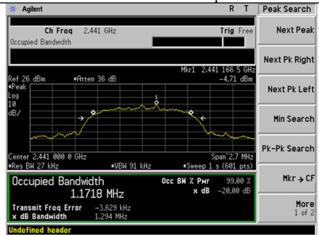
3DH1 2441 MHz -20dB Occupied Bandwidth
