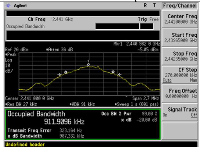
DH1 2441 MHz -20dB Occupied Bandwidth
