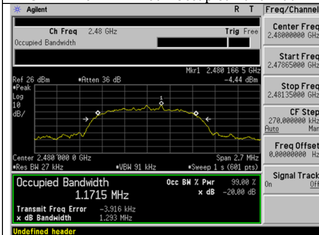
3DH1 2480 MHz -20dB Occupied Bandwidth
