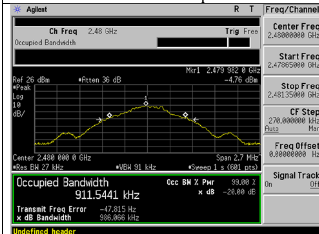
DH1 2480 MHz -20dB Occupied Bandwidth
