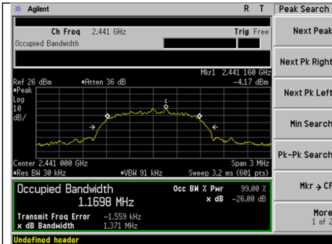
3DH1 2441 MHz 99 Percent Occupied Bandwidth
