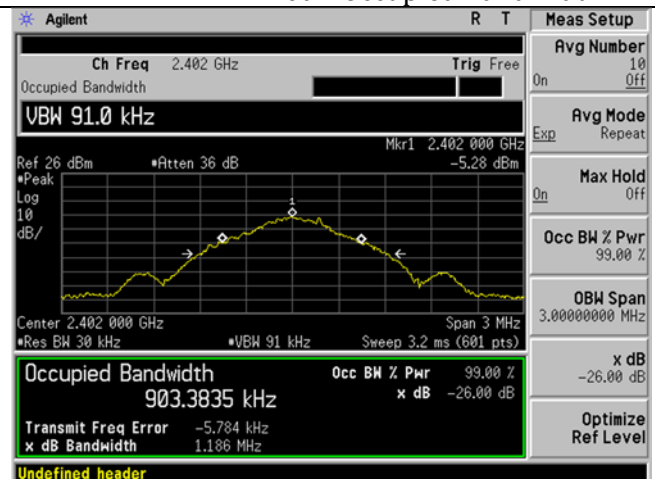
DH1 2402 MHz 99 Percent Occupied Bandwidth
