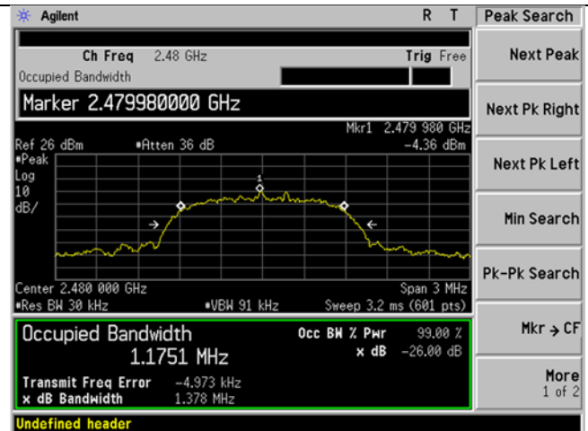
3DH1 2480 MHz 99 Percent Occupied Bandwidth
