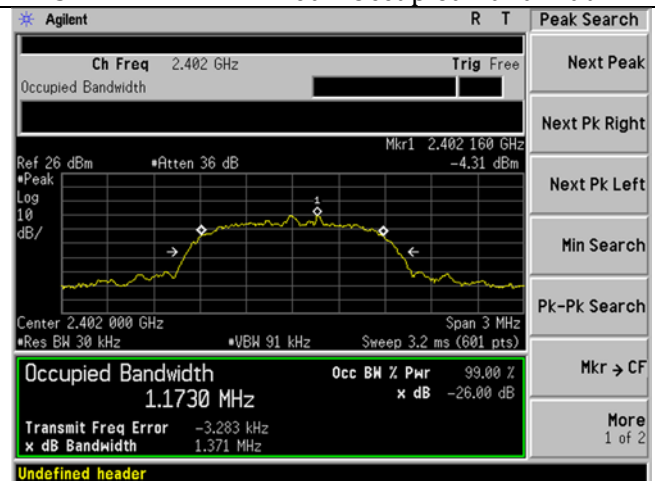
3DH1 2402 MHz 99 Percent Occupied Bandwidth
