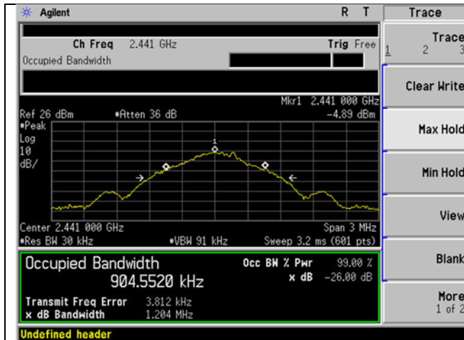
DH1 2441 MHz 99 Percent Occupied Bandwidth
