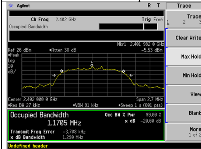
3DH1 2402 MHz -20dB Occupied Bandwidth
