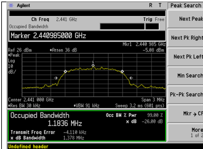
2DH1 2441 MHz 99 Percent Occupied Bandwidth
