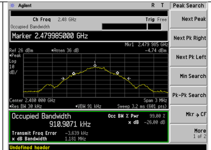
DH1 2480 MHz 99 Percent Occupied Bandwidth
