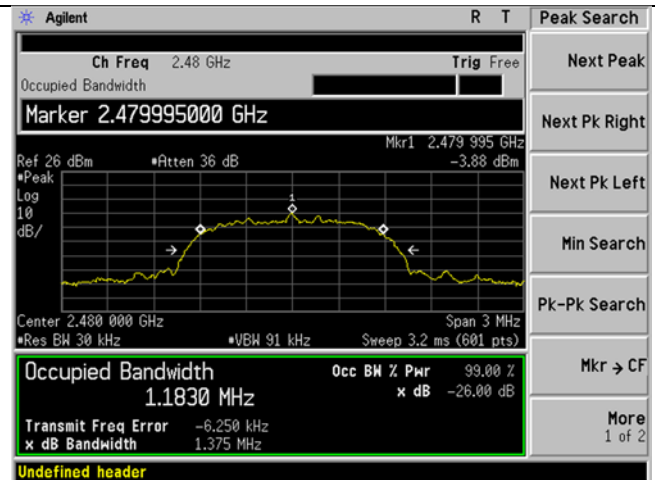
2DH1 2480 MHz 99 Percent Occupied Bandwidth
