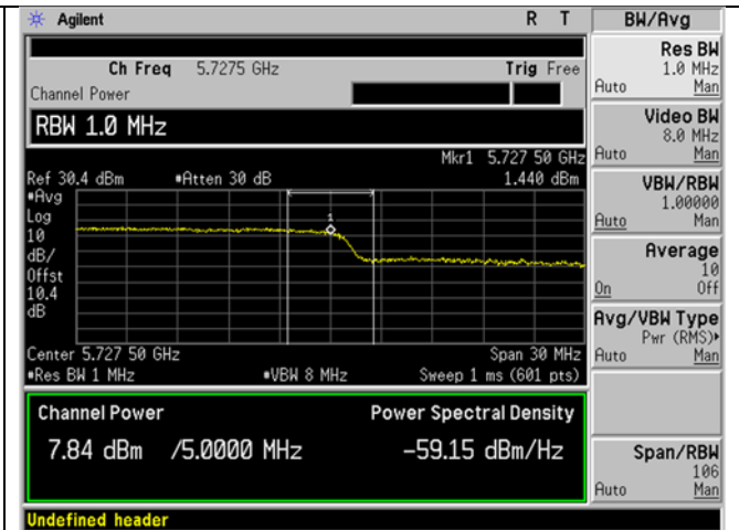
n40mode 5710 MHz straddle power right
