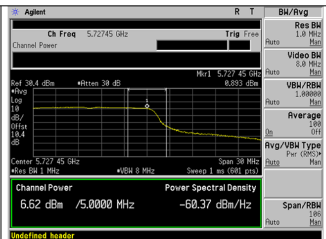
a-mode 5720 MHz straddle power right
