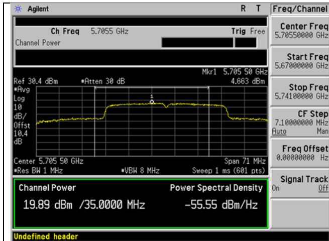
n40mode 5710 MHz straddle power left
