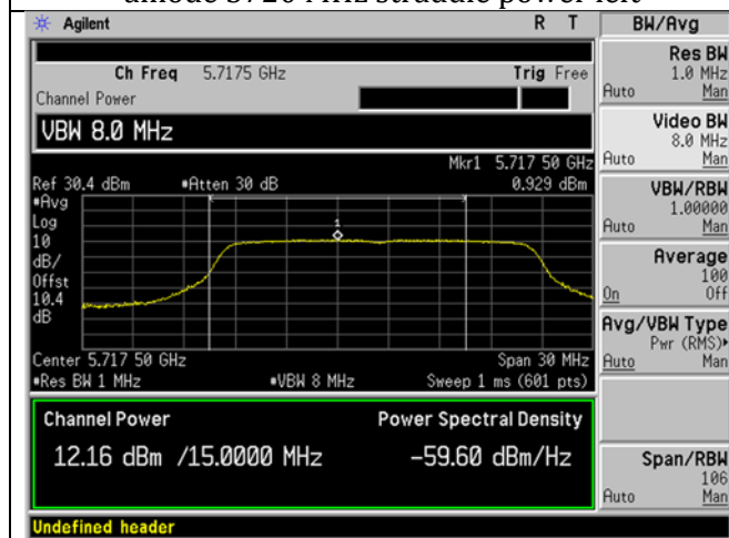
n20mode 5720 MHz straddle power left
