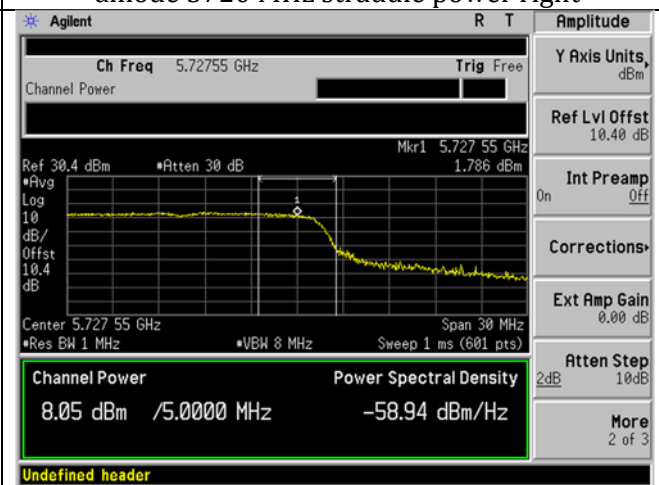
n20mode 5720 MHz straddle power right
