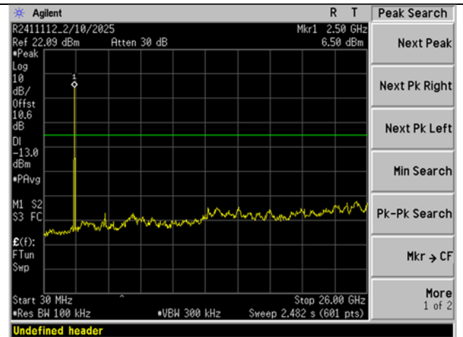
BLE_High Ch_2480MHz_1MBit_-20dBc_30MHz- 26GHz
