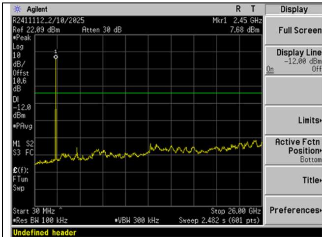
BLE_High Ch_2442MHz_2MBit_-20dBc_30MHz- 26GHz
