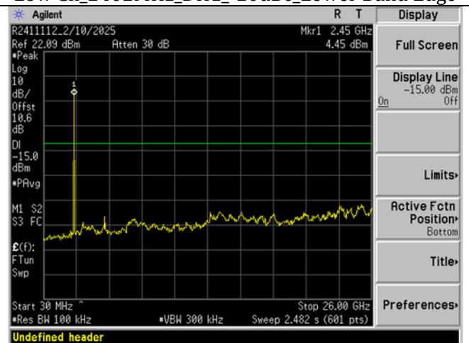
Mid Ch_2441MHz_3DH1_-20dBc_30-26GHz
