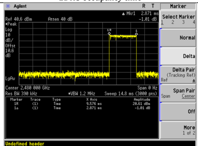
3DH5 occupancy time
