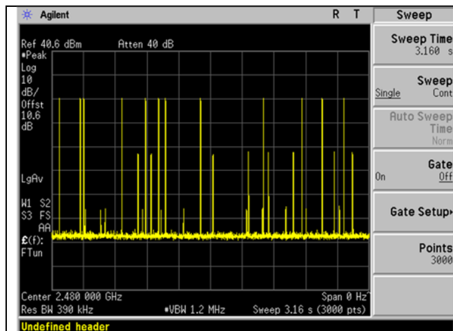
2DH5 observation period 3.16sec
