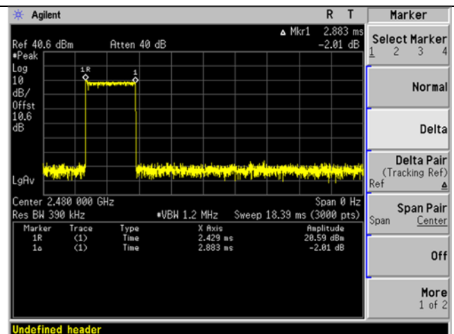
2DH5 occupancy time
