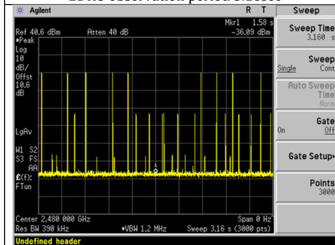
3DH5 observed period 3.16sec
