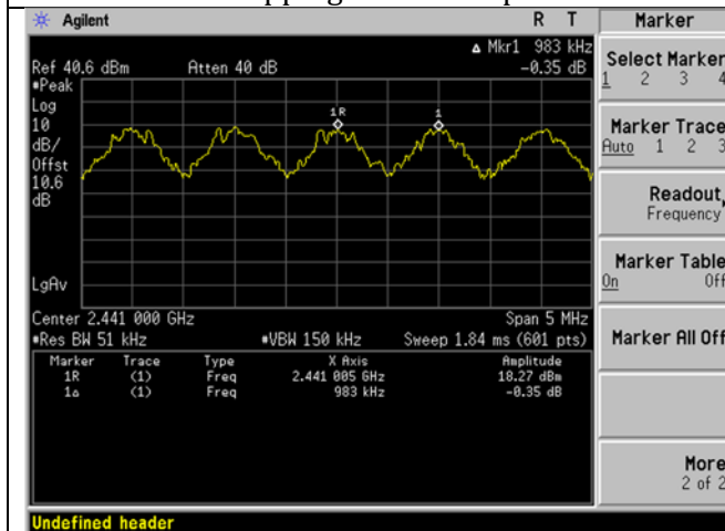
DH5 Hopping Channel Separation
