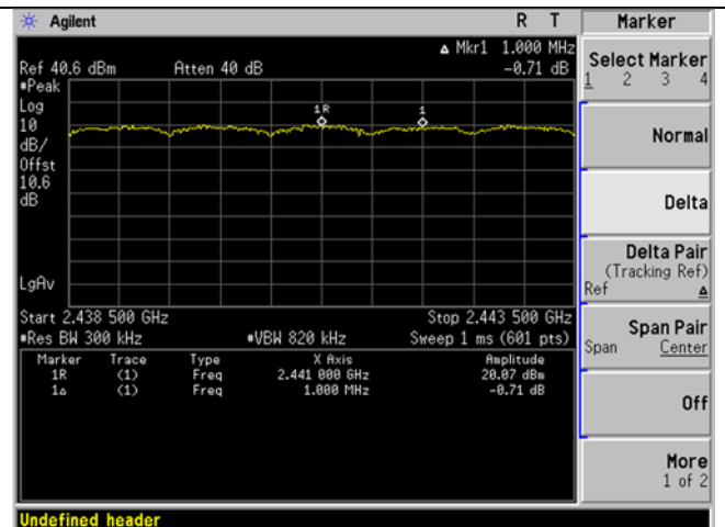
3DH5 Hopping Channel Separation
