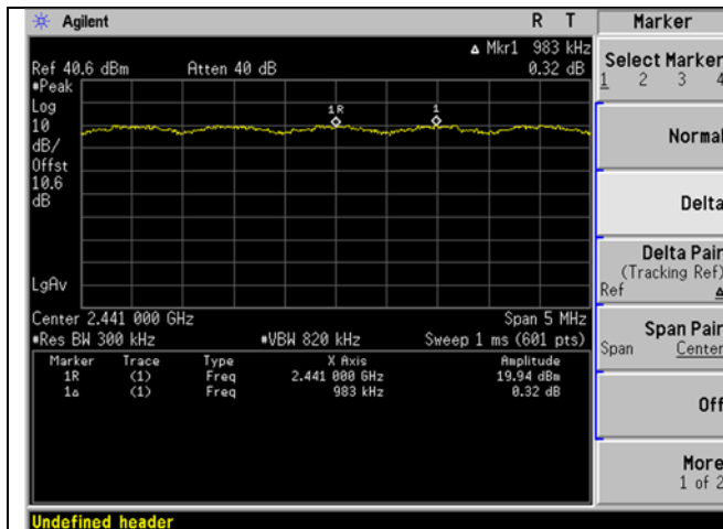
2DH5 Hopping Channel Separation
