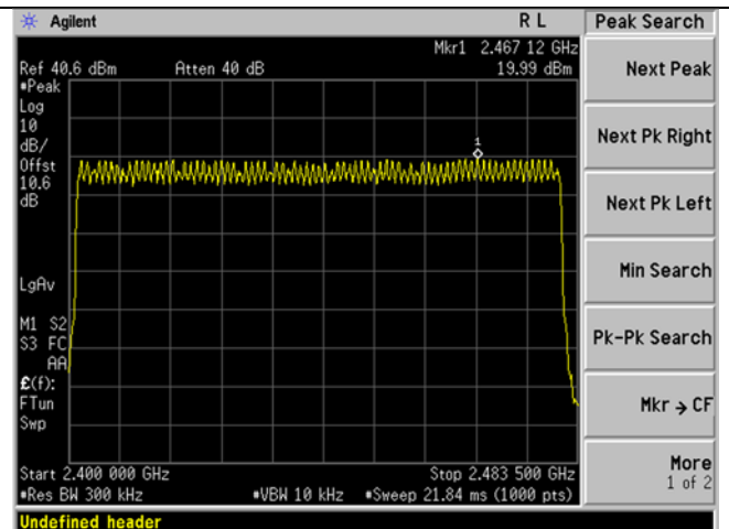
2DH5 Number of Hopping Channel
