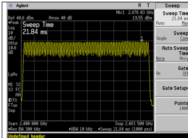
DH5 Number of Hopping Channel
