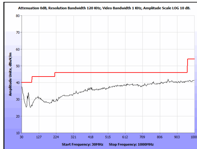
Plot 11. Radiated Spurious Emissions, Mid Channel, 2442 MHz, 802.11g, 30 MHz – 1 GHz, Average
