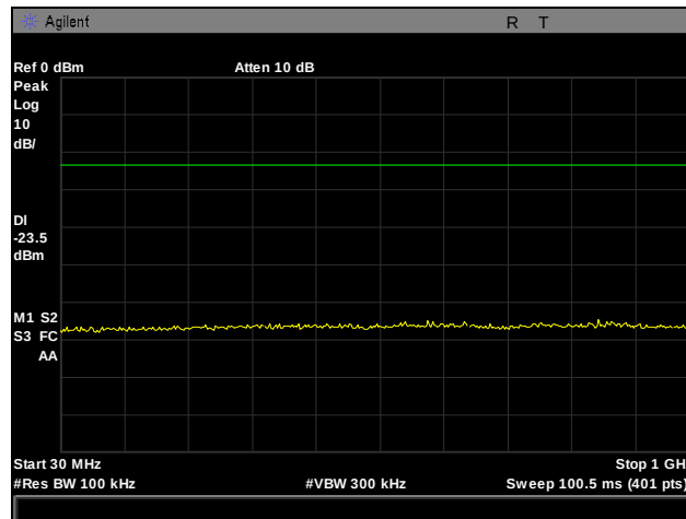
Plot 27. Conducted Spurious Emissions, High Channel, 2462 MHz, 802.11g, 30 MHz – 1 GHz
