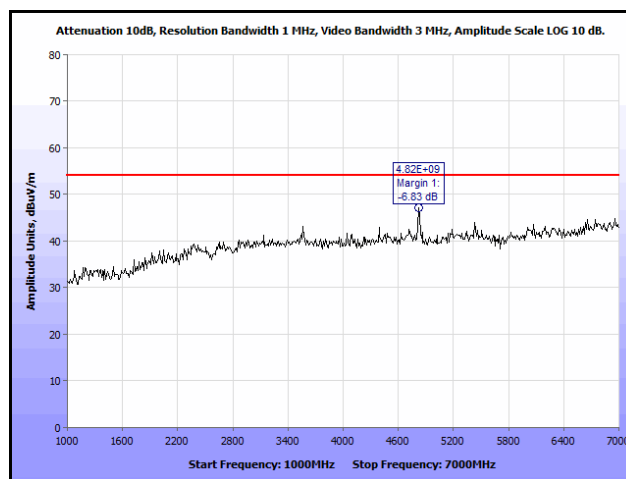
Plot 9. Radiated Spurious Emissions, Low Channel, 2412 MHz, 802.11g, 1 GHz – 7 GHz, Average
