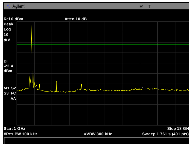
Plot 24. Conducted Spurious Emissions, Low Channel, 2412 MHz, 802.11g, 1 GHz – 18 GHz
