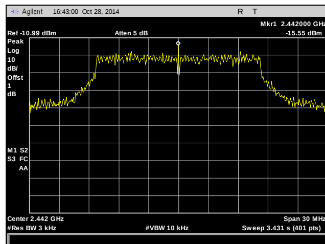
Plot 32. Peak Power Spectral Density, Mid Channel, 2442 MHz, 802.11g
