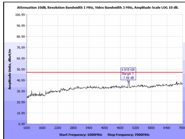
Plot 17. Radiated Spurious Emissions, High Channel, 2462 MHz, 802.11g, 1 GHz – 7 GHz, Average
