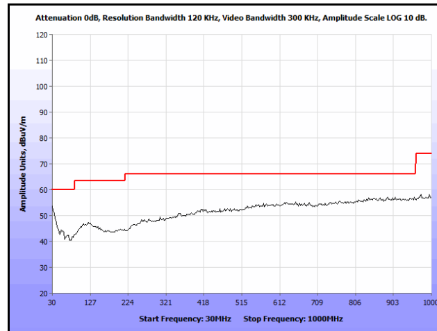
Plot 16. Radiated Spurious Emissions, High Channel, 2462 MHz, 802.11g, 30 MHz – 1 GHz, Peak
