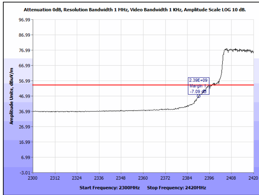
Plot 19. Radiated Band Edge, 802.11g, Channel 1, Average
