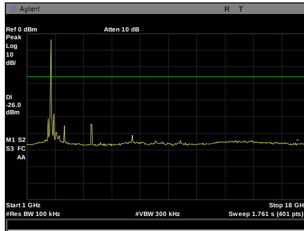
Plot 26. Conducted Spurious Emissions, Mid Channel, 2442 MHz, 802.11g, 1 GHz – 18 GHz
