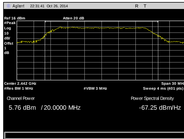
Plot 5. Peak Power Output, Mid Channel, 2442 MHz, 802.11g
