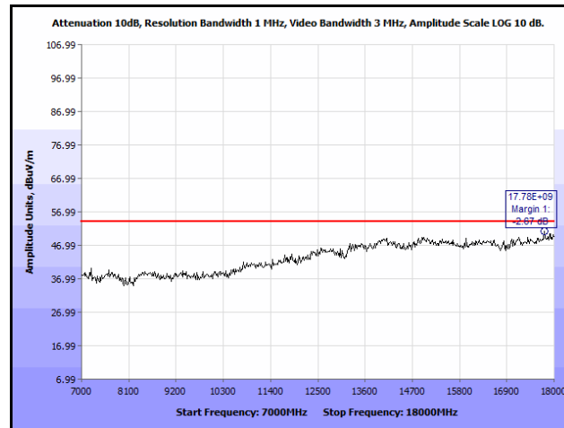
Plot 10. Radiated Spurious Emissions, Low Channel, 2412 MHz, 802.11g, 7 GHz – 18 GHz, Average
