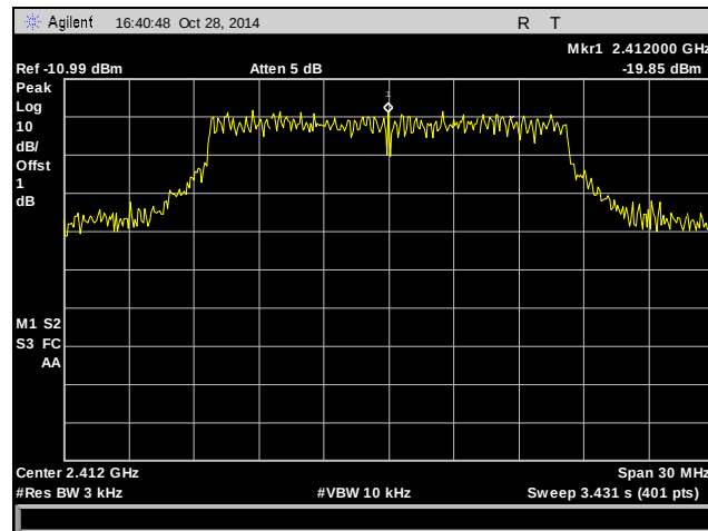
Plot 31. Peak Power Spectral Density, Low Channel, 2412 MHz, 802.11g
