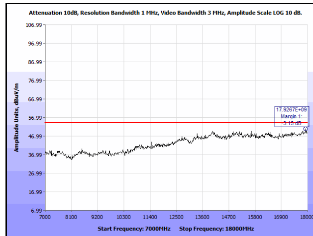
Plot 14. Radiated Spurious Emissions, Mid Channel, 2442 MHz, 802.11g, 7 GHz – 18 GHz, Average
