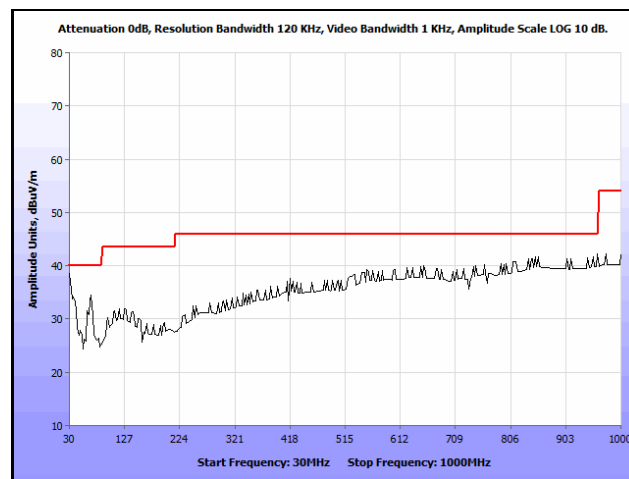
Plot 15. Radiated Spurious Emissions, High Channel, 2462 MHz, 802.11g, 30 MHz – 1 GHz, Average
