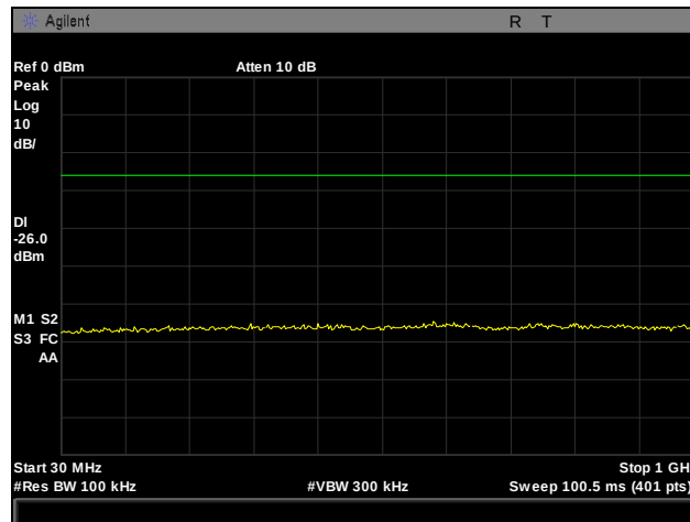
Plot 25. Conducted Spurious Emissions, Mid Channel, 2442 MHz, 802.11g, 30 MHz – 1 GHz
