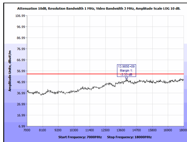
Plot 18. Radiated Spurious Emissions, High Channel, 2462 MHz, 802.11g, 7 GHz – 18 GHz, Average
