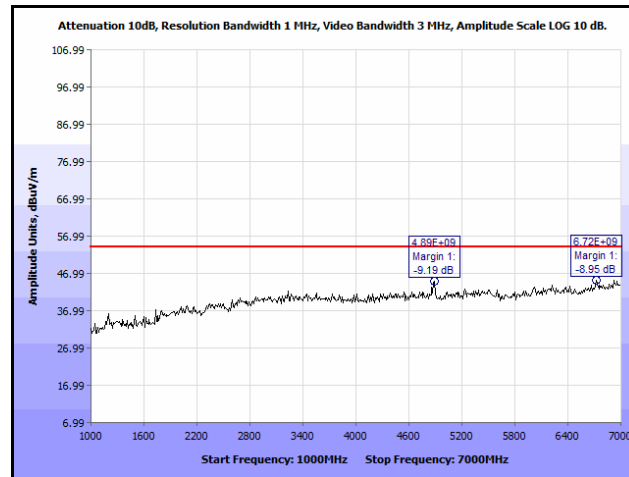
Plot 13. Radiated Spurious Emissions, Mid Channel, 2442 MHz, 802.11g, 1 GHz – 7 GHz, Average
