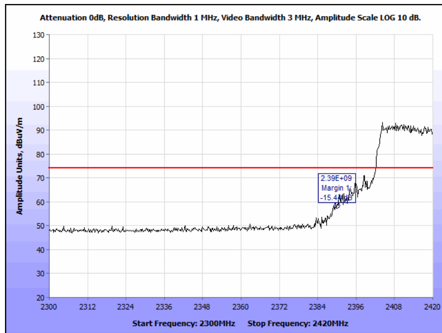
Plot 20. Radiated Band Edge, 802.11g, Channel 1, Peak
