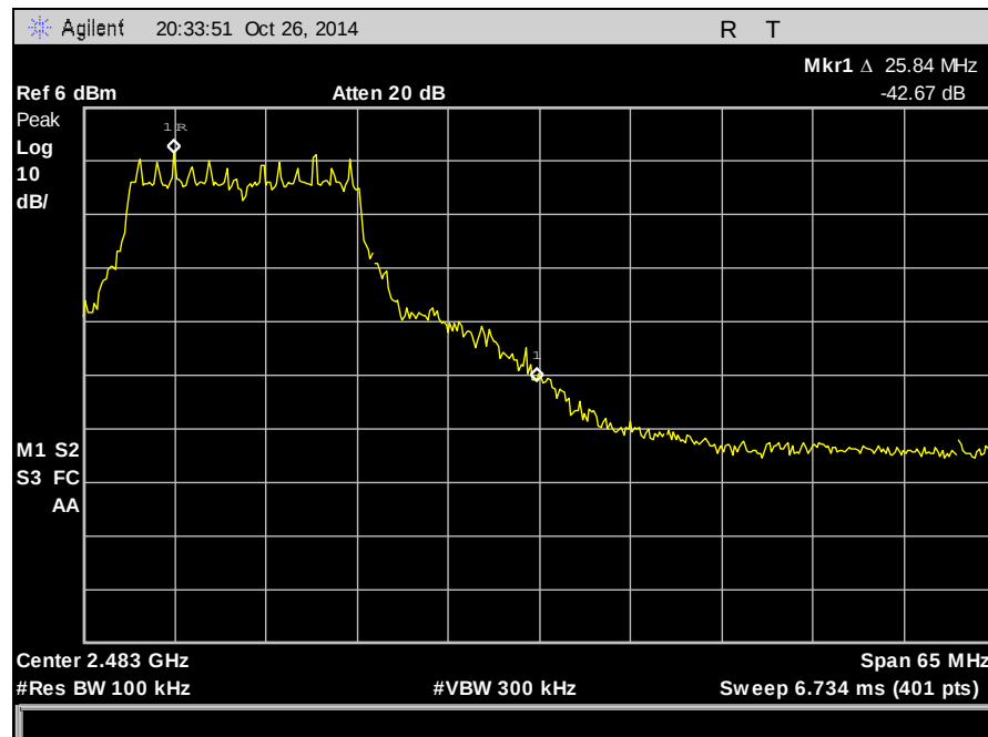
Plot 30. Conducted Band Edge, High Channel, 2462 MHz, 802.11g
