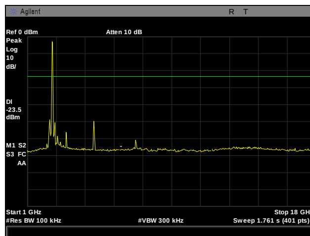
Plot 28. Conducted Spurious Emissions, High Channel, 2462 MHz, 802.11g, 1 GHz – 18 GHz
