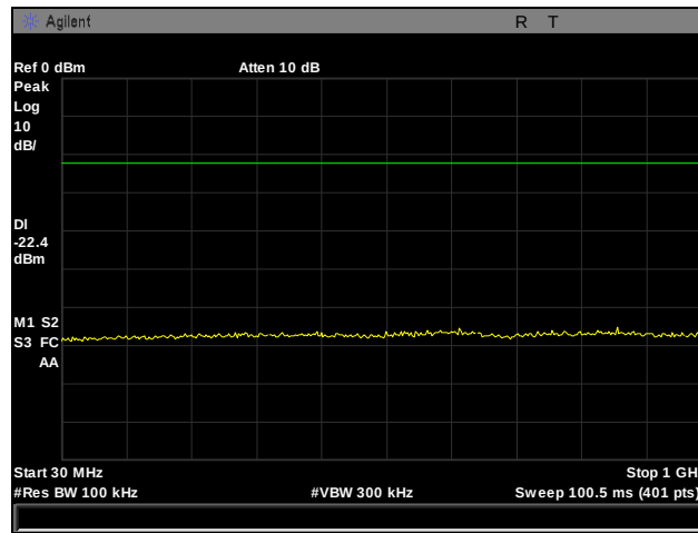
Plot 23. Conducted Spurious Emissions, Low Channel, 2412 MHz, 802.11g, 30 MHz – 1 GHz
