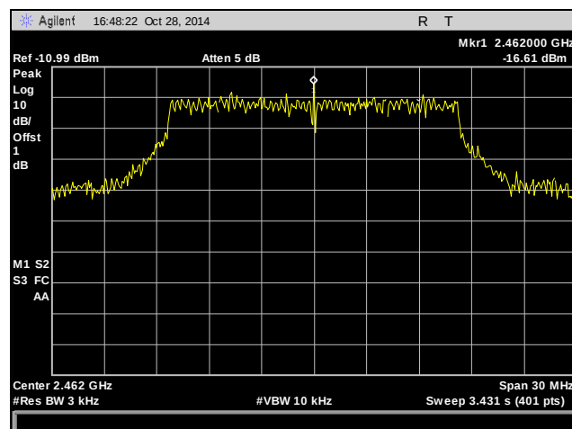
Plot 33. Peak Power Spectral Density, High Channel, 2462 MHz, 802.11g
