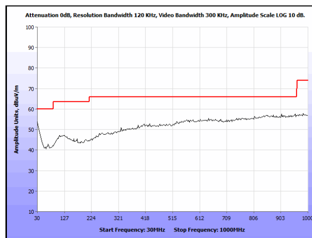
Plot 12. Radiated Spurious Emissions, Mid Channel, 2442 MHz, 802.11g, 30 MHz – 1 GHz, Peak
