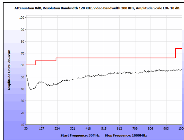
Plot 8. Radiated Spurious Emissions, Low Channel, 2412 MHz, 802.11g, 30 MHz – 1 GHz, Peak
