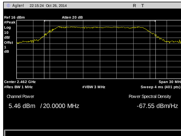
Plot 6. Peak Power Output, High Channel, 2462 MHz, 802.11g
