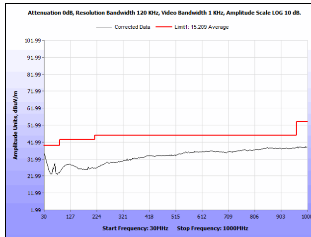
Plot 7. Radiated Spurious Emissions, Low Channel, 2412 MHz, 802.11g, 30 MHz – 1 GHz, Average
