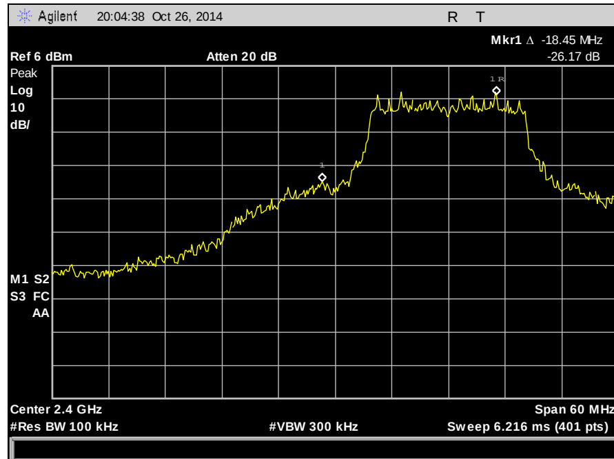
Plot 29. Conducted Band Edge, Low Channel, 2412 MHz, 802.11g
