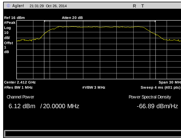
Plot 4. Peak Power Output, Low Channel, 2412 MHz, 802.11g
