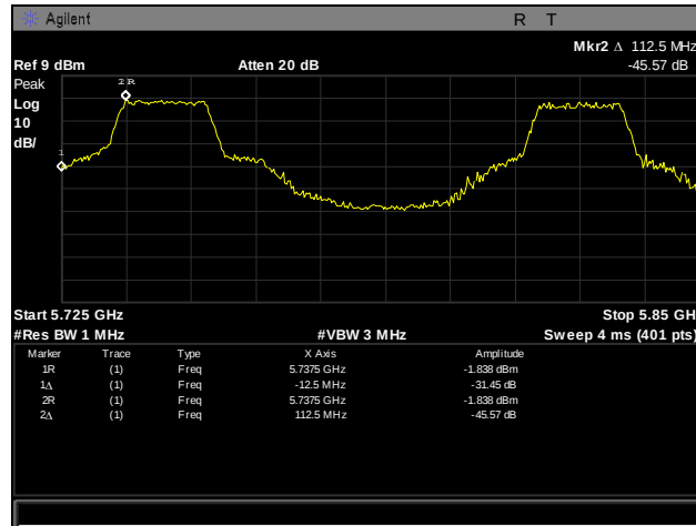
Plot 78. Frequency Stability, 5725-5850 MHz, 55°C, 120°C
