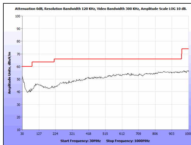
Plot 46. Radiated Spurious Emissions, High Channel, 5825 MHz, 802.11a, 30 MHz – 1 GHz, Peak
