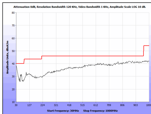
Plot 25. Radiated Spurious Emissions, Mid Channel, 5220 MHz, 802.11a, 30 MHz – 1 GHz, Average
