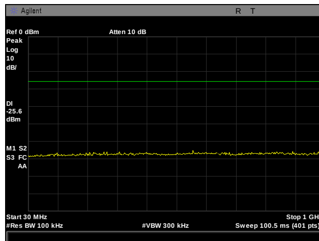
Plot 48. Conducted Spurious Emissions, Mid Channel, 2442 MHz, 802.11b, 30 MHz – 1 GHz
