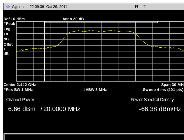
Plot 9. Peak Power Output, Mid Channel, 2442 MHz, 802.11b
