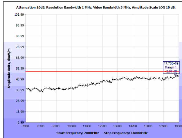
Plot 29. Radiated Spurious Emissions, Low Channel, 2412 MHz, 802.11g, 7 GHz – 18 GHz, Average
