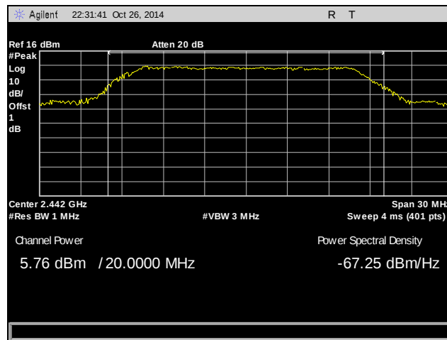
Plot 12. Peak Power Output, Mid Channel, 2442 MHz, 802.11g
