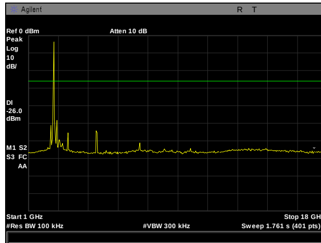
Plot 55. Conducted Spurious Emissions, Mid Channel, 2442 MHz, 802.11g, 1 GHz – 18 GHz
