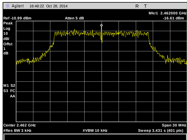
Plot 66. Peak Power Spectral Density, High Channel, 2462 MHz, 802.11g
