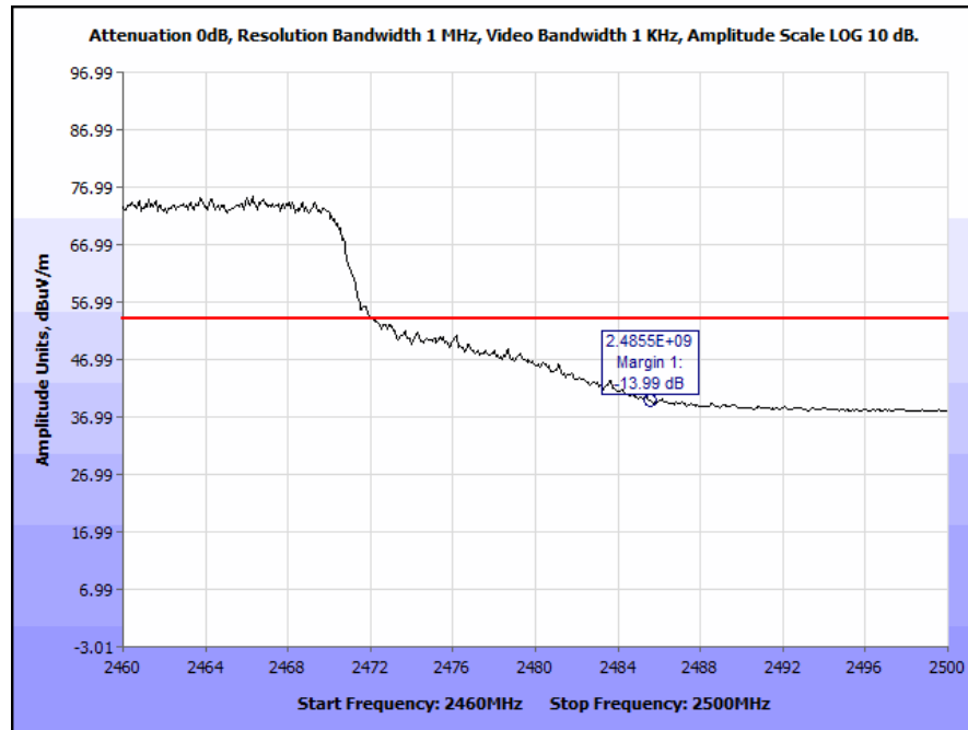
Plot 43. Radiated Band Edge, 802.11g, Channel 11, Average
