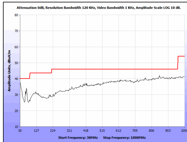
Plot 29. Radiated Spurious Emissions, Mid Channel, 2442 MHz, 802.11g, 30 MHz – 1 GHz, Average
