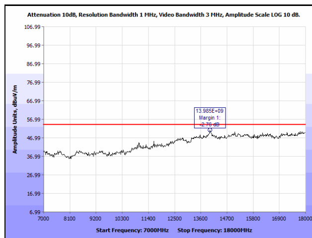
Plot 16. Radiated Spurious Emissions, Low Channel, 2412 MHz, 802.11b, 7 GHz – 18 GHz, Average
