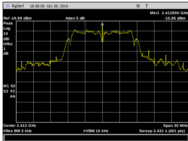
Plot 61. Peak Power Spectral Density, Low Channel, 2412 MHz, 802.11b
