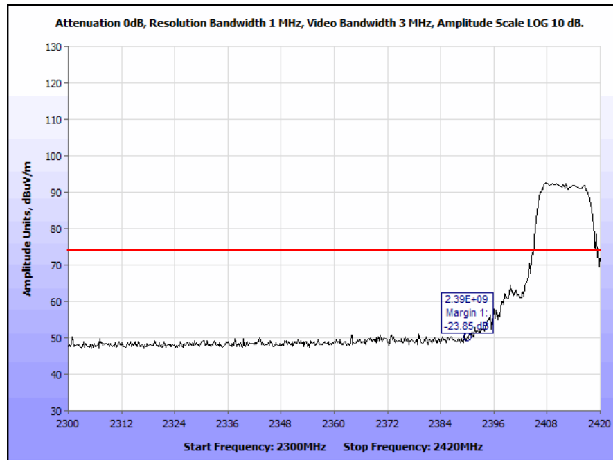
Plot 38. Radiated Band Edge, 802.11b, Channel 1, Peak
