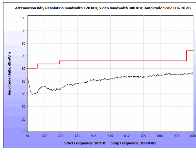
Plot 26. Radiated Spurious Emissions, Low Channel, 2412 MHz, 802.11g, 30 MHz – 1 GHz, Peak
