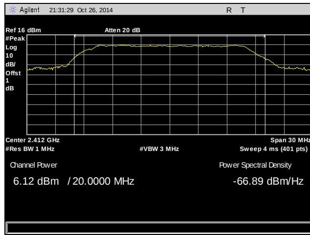
Plot 10. Peak Power Output, Low Channel, 2412 MHz, 802.11g
