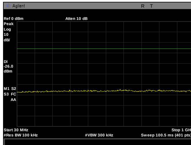
Plot 53. Conducted Spurious Emissions, Mid Channel, 2442 MHz, 802.11g, 30 MHz – 1 GHz
