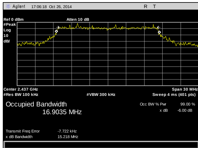
Plot 5. Occupied Bandwidth, Mid Channel, 2437 MHz, 802.11g
