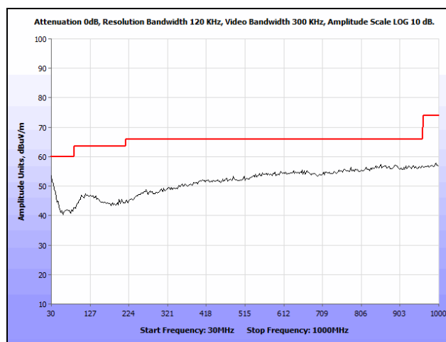
Plot 18. Radiated Spurious Emissions, Mid Channel, 2442 MHz, 802.11b, 30 MHz – 1 GHz, Peak
