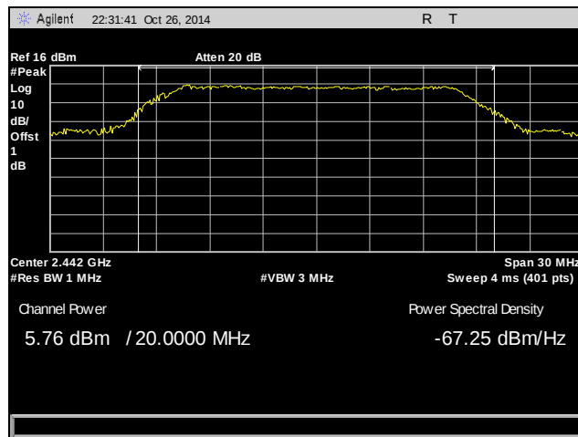
Plot 11. Peak Power Output, Mid Channel, 2442 MHz, 802.11g
