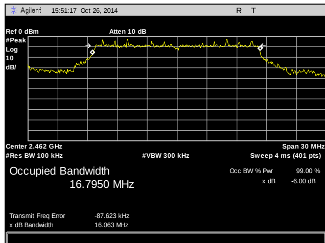
Plot 6. Occupied Bandwidth, High Channel, 2462 MHz, 802.11g
