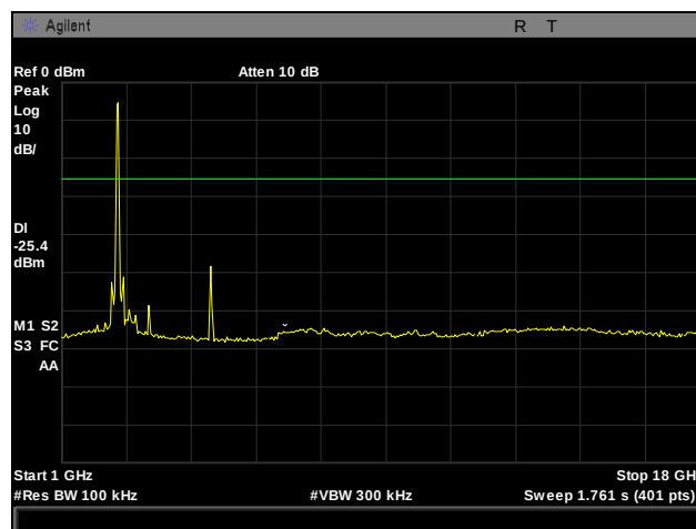
Plot 50. Conducted Spurious Emissions, High Channel, 2462 MHz, 802.11b, 1 GHz – 18 GHz
