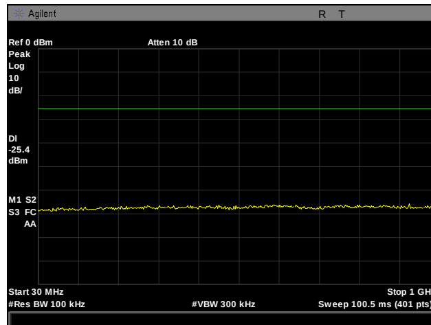
Plot 49. Conducted Spurious Emissions, High Channel, 2462 MHz, 802.11b, 30 MHz – 1 GHz
