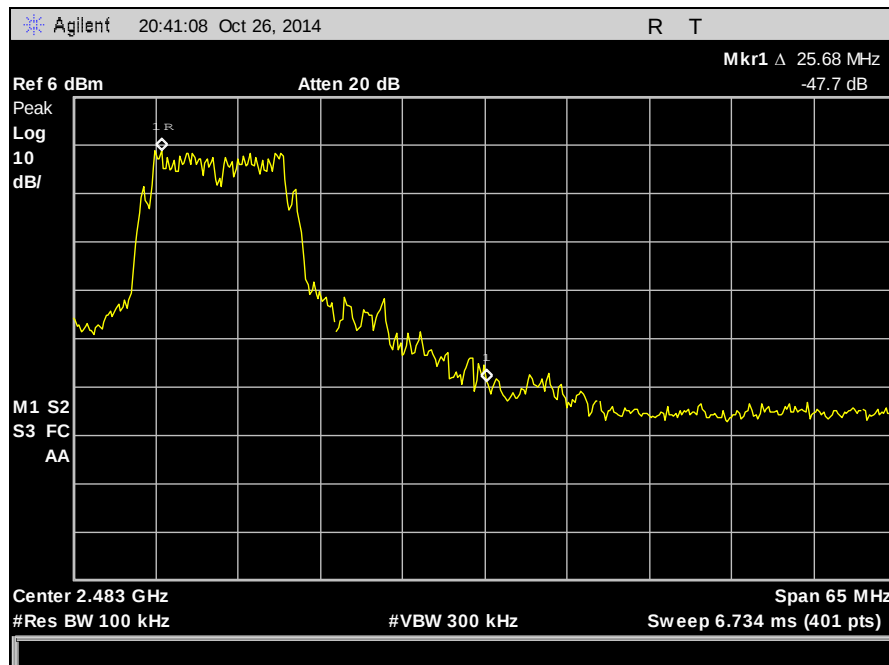
Plot 58. Conducted Band Edge, High Channel, 2462 MHz, 802.11b
