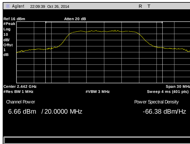
Plot 8. Peak Power Output, Mid Channel, 2442 MHz, 802.11b
