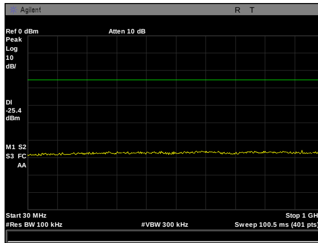
Plot 45. Conducted Spurious Emissions, Low Channel, 2412 MHz, 802.11b, 30 MHz – 1 GHz
