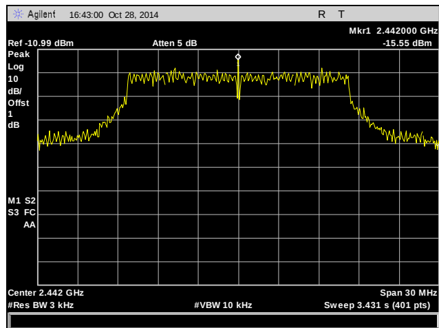
Plot 65. Peak Power Spectral Density, Mid Channel, 2442 MHz, 802.11g
