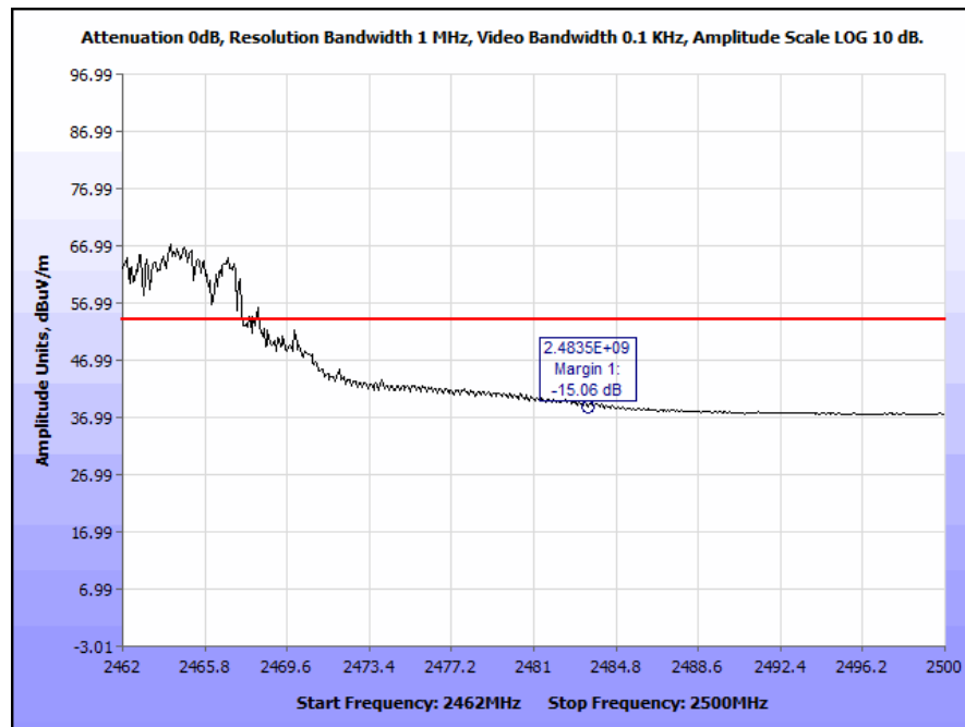
Plot 39. Radiated Band Edge, 802.11b, Channel 11, Average
