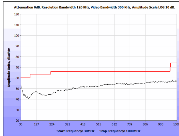
Plot 34. Radiated Spurious Emissions, High Channel, 2462 MHz, 802.11g, 30 MHz – 1 GHz, Peak
