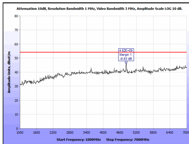
Plot 27. Radiated Spurious Emissions, Low Channel, 2412 MHz, 802.11g, 1 GHz – 7 GHz, Average
