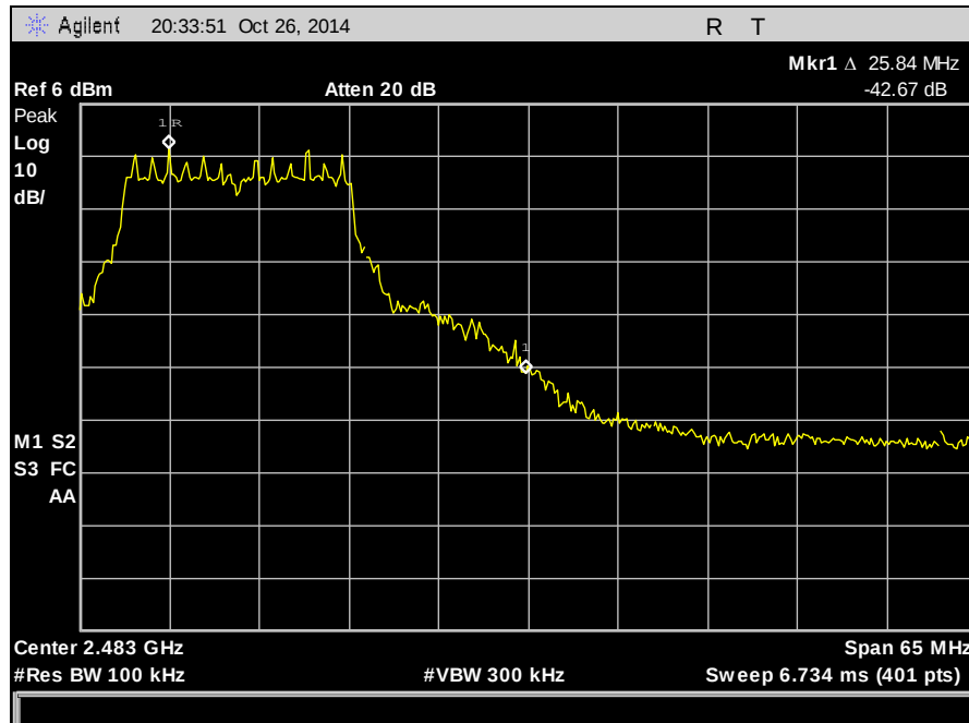
Plot 60. Conducted Band Edge, High Channel, 2462 MHz, 802.11g
