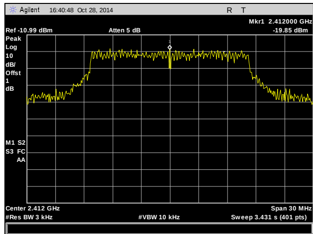
Plot 64. Peak Power Spectral Density, Low Channel, 2412 MHz, 802.11g
