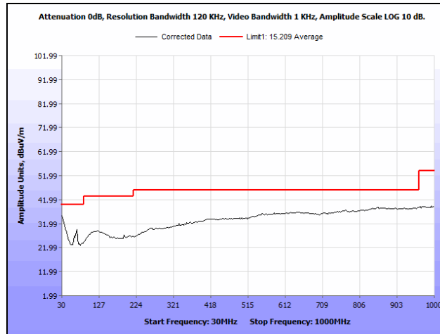
Plot 25. Radiated Spurious Emissions, Low Channel, 2412 MHz, 802.11g, 30 MHz – 1 GHz, Average
