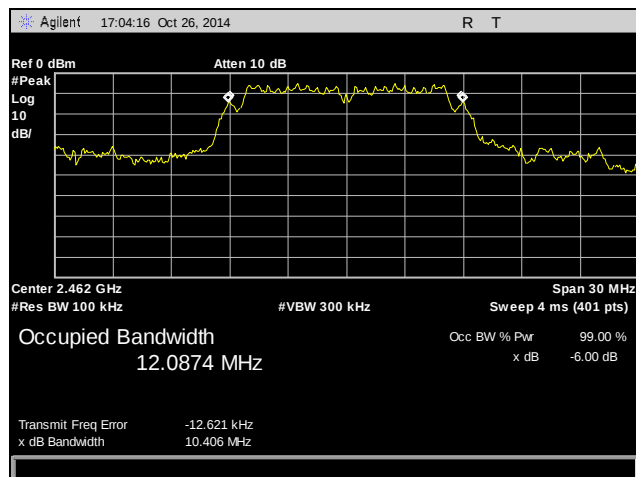
Plot 3. Occupied Bandwidth, High Channel, 2462 MHz, 802.11b
