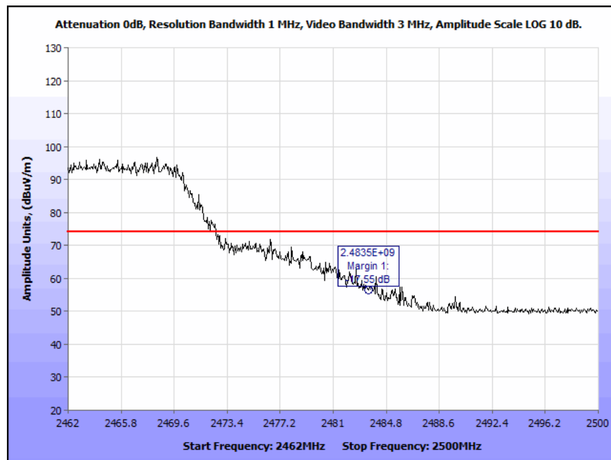
Plot 40. Radiated Band Edge, 802.11b, Channel 11, Peak
