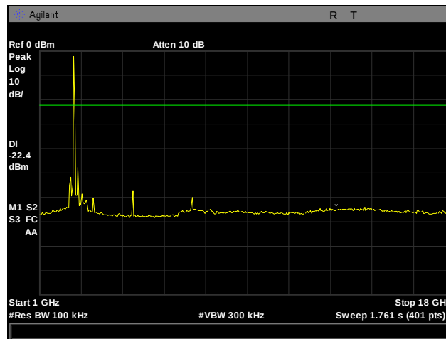
Plot 52. Conducted Spurious Emissions, Low Channel, 2412 MHz, 802.11g, 1 GHz – 18 GHz
