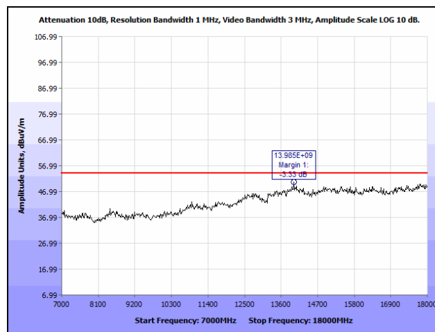
Plot 36. Radiated Spurious Emissions, High Channel, 2462 MHz, 802.11g, 7 GHz – 18 GHz, Average
