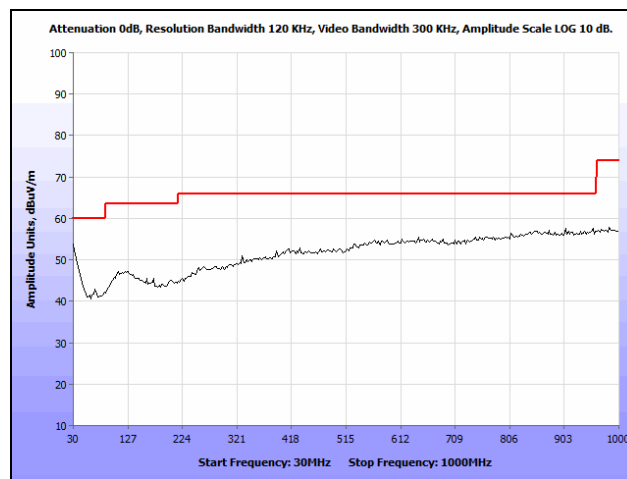
Plot 30. Radiated Spurious Emissions, Mid Channel, 2442 MHz, 802.11g, 30 MHz – 1 GHz, Peak
