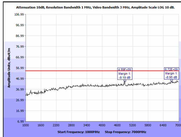
Plot 31. Radiated Spurious Emissions, Mid Channel, 2442 MHz, 802.11g, 1 GHz – 7 GHz, Average
