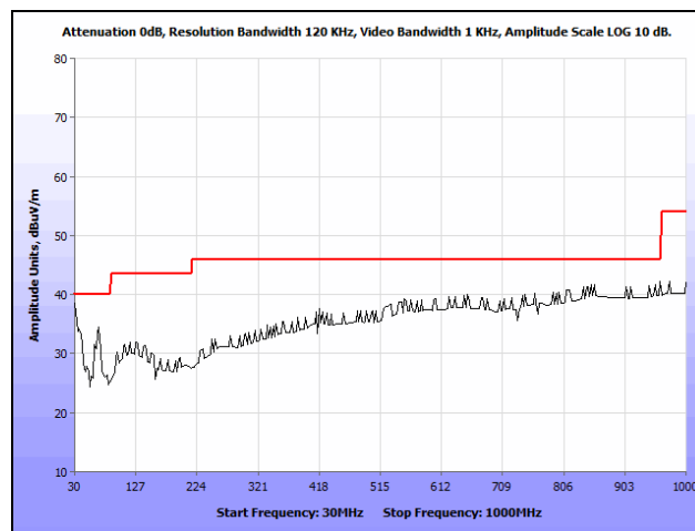
Plot 33. Radiated Spurious Emissions, High Channel, 2462 MHz, 802.11g, 30 MHz – 1 GHz, Average
