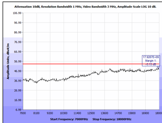
Plot 32. Radiated Spurious Emissions, Mid Channel, 2442 MHz, 802.11g, 7 GHz – 18 GHz, Average
