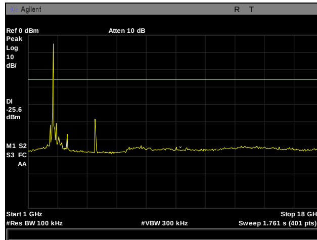
Plot 48. Conducted Spurious Emissions, Mid Channel, 2442 MHz, 802.11b, 1 GHz – 18 GHz
