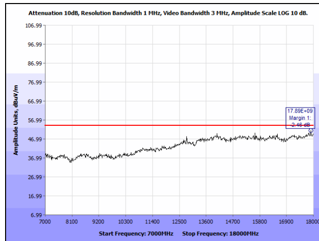
Plot 20. Radiated Spurious Emissions, Mid Channel, 2442 MHz, 802.11b, 7 GHz – 18 GHz, Average
