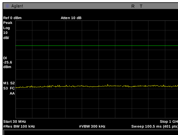
Plot 47. Conducted Spurious Emissions, Mid Channel, 2442 MHz, 802.11b, 30 MHz – 1 GHz
