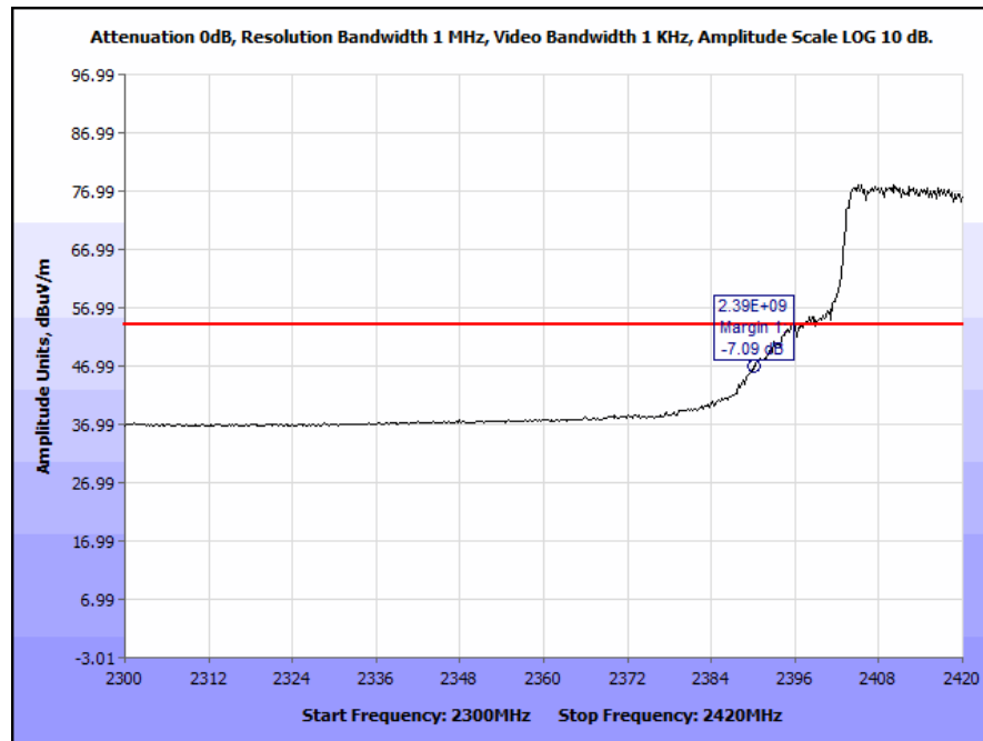
Plot 41. Radiated Band Edge, 802.11g, Channel 1, Average
