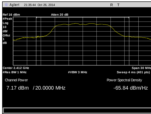
Plot 7. Peak Power Output, Low Channel, 2412 MHz, 802.11b
