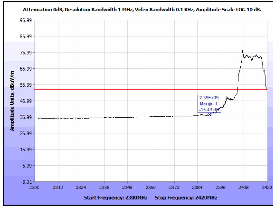
Plot 37. Radiated Band Edge, 802.11b, Channel 1, Average
