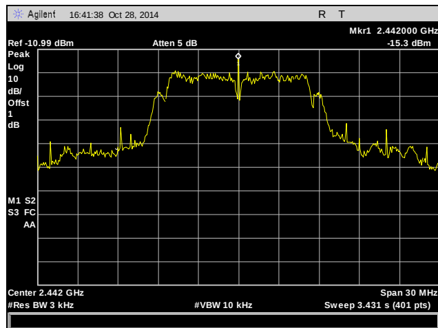
Plot 62. Peak Power Spectral Density, Mid Channel, 2442 MHz, 802.11b
