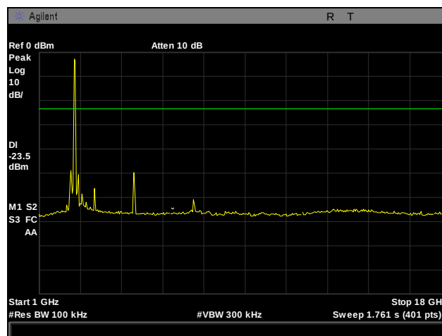
Plot 56. Conducted Spurious Emissions, High Channel, 2462 MHz, 802.11g, 1 GHz – 18 GHz
