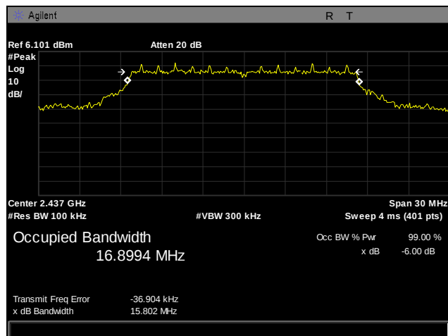
Plot 2. Occupied Bandwidth, Mid Channel, 2437 MHz, 802.11b
