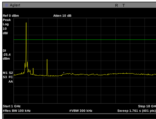
Plot 46. Conducted Spurious Emissions, Low Channel, 2412 MHz, 802.11b, 1 GHz – 18 GHz
