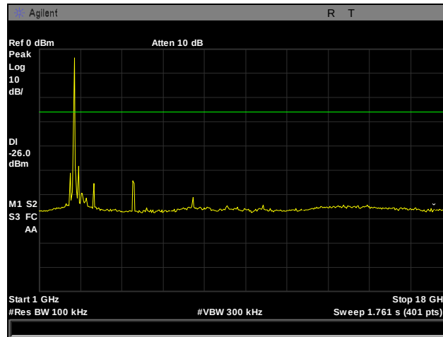
Plot 54. Conducted Spurious Emissions, Mid Channel, 2442 MHz, 802.11g, 1 GHz – 18 GHz
