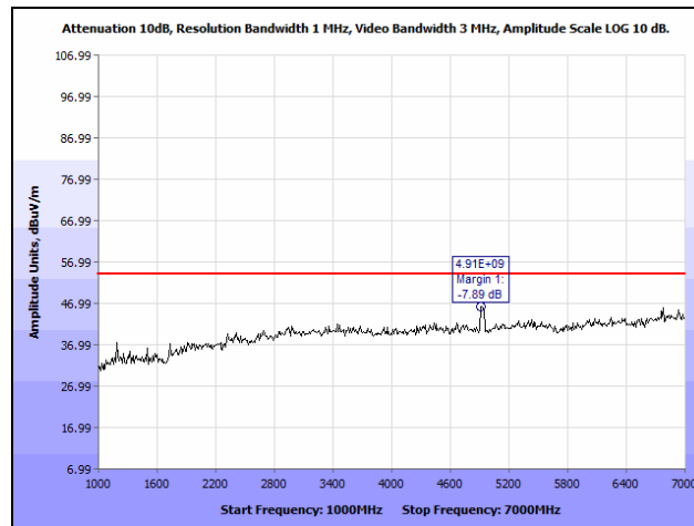
Plot 35. Radiated Spurious Emissions, High Channel, 2462 MHz, 802.11g, 1 GHz – 7 GHz, Average
