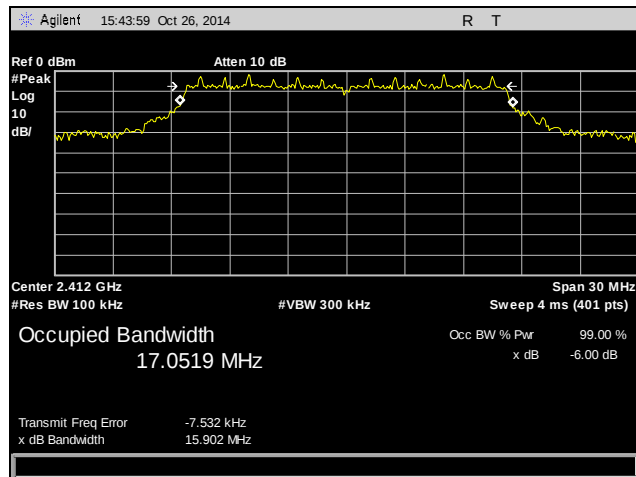
Plot 4. Occupied Bandwidth, Low Channel, 2412 MHz, 802.11g
