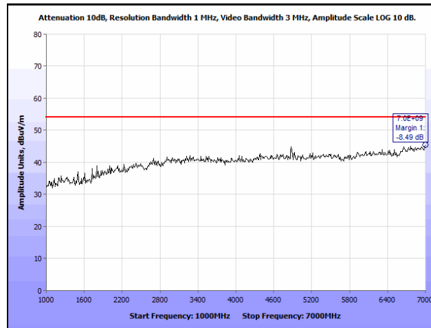
Plot 19. Radiated Spurious Emissions, Mid Channel, 2442 MHz, 802.11b, 1 GHz – 7 GHz, Average
