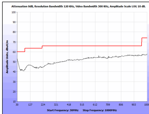
Plot 14. Radiated Spurious Emissions, Low Channel, 2412 MHz, 802.11b, 30 MHz – 1 GHz, Peak
