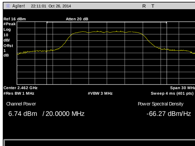
Plot 9. Peak Power Output, High Channel, 2462 MHz, 802.11b
