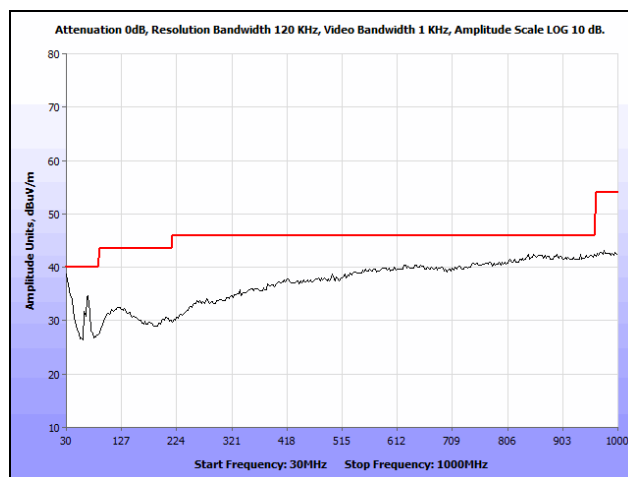
Plot 17. Radiated Spurious Emissions, Mid Channel, 2442 MHz, 802.11b, 30 MHz – 1 GHz, Average
