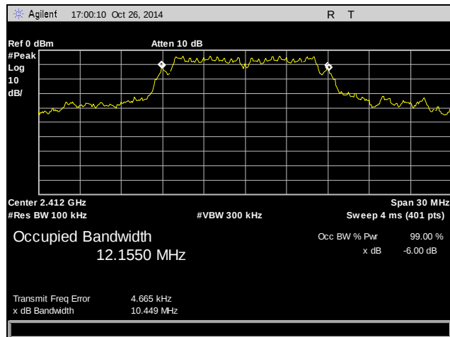
Plot 1. Occupied Bandwidth, Low Channel, 2412 MHz, 802.11b
