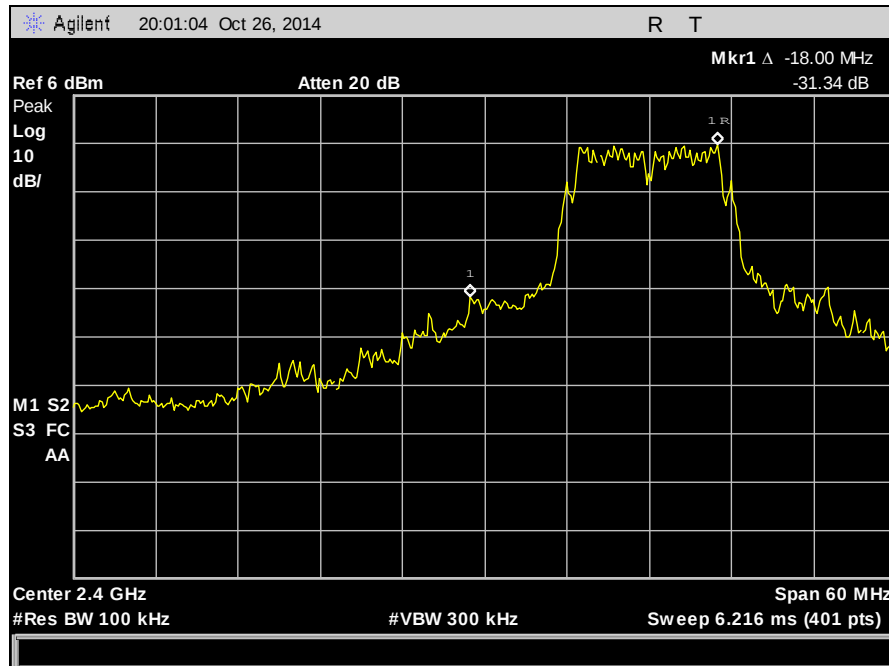
Plot 57. Conducted Band Edge, Low Channel, 2412 MHz, 802.11b
