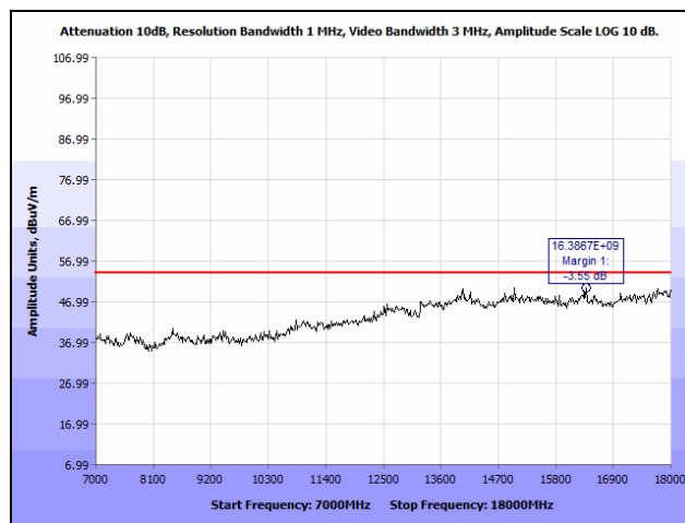
Plot 24. Radiated Spurious Emissions, High Channel, 2462 MHz, 802.11b, 7 GHz – 18 GHz, Average
