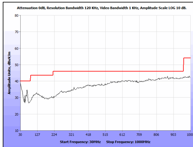
Plot 13. Radiated Spurious Emissions, Low Channel, 2412 MHz, 802.11b, 30 MHz – 1 GHz, Average
