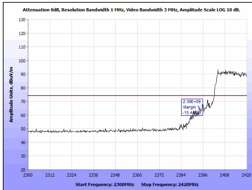
Plot 42. Radiated Band Edge, 802.11g, Channel 1, Peak
