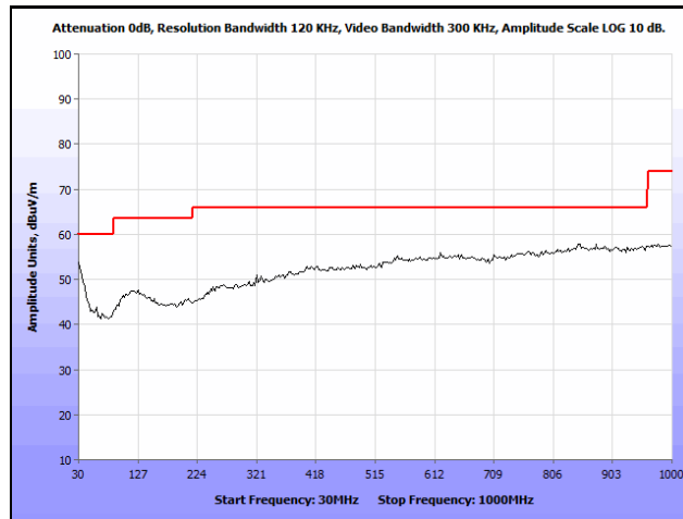
Plot 22. Radiated Spurious Emissions, High Channel, 2462 MHz, 802.11b, 30 MHz – 1 GHz, Peak
