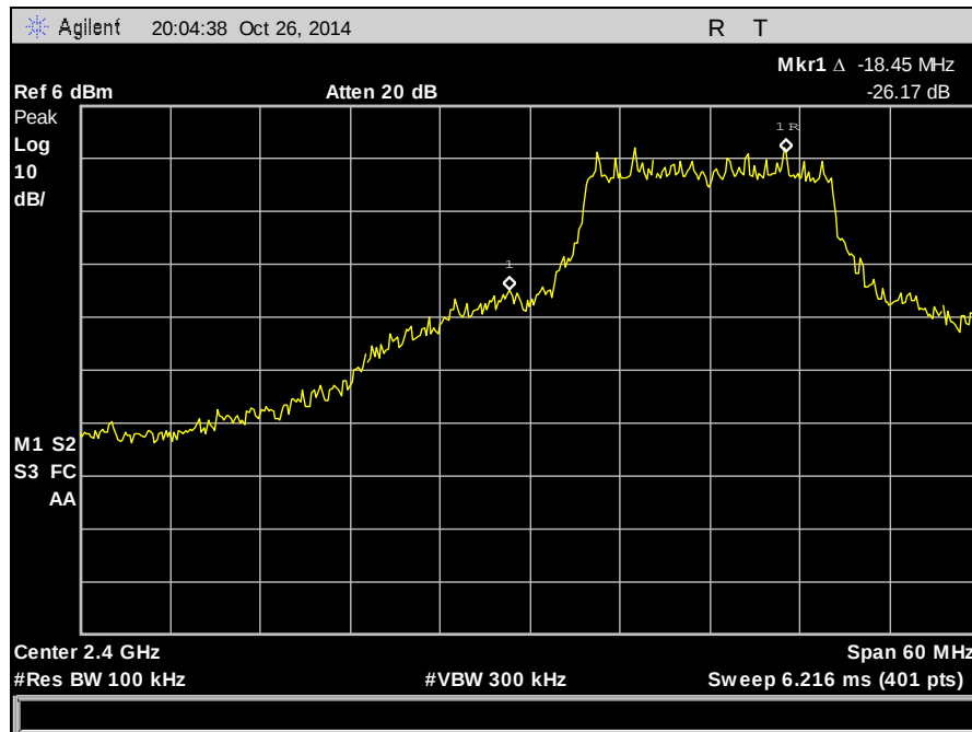
Plot 59. Conducted Band Edge, Low Channel, 2412 MHz, 802.11g
