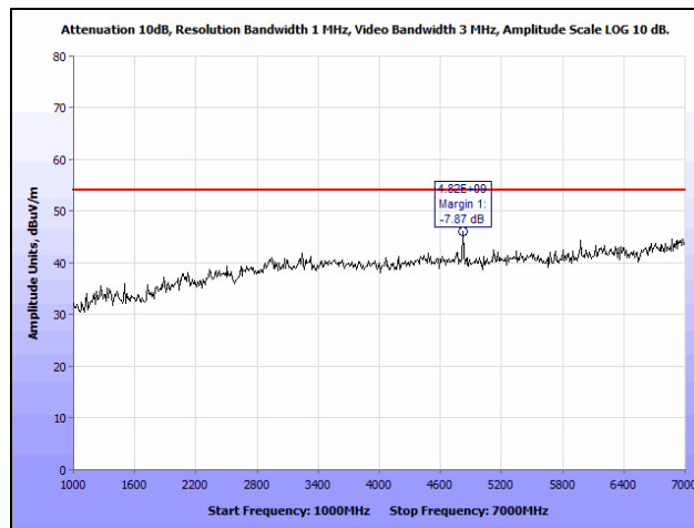
Plot 15. Radiated Spurious Emissions, Low Channel, 2412 MHz, 802.11b, 1 GHz – 7 GHz, Average
