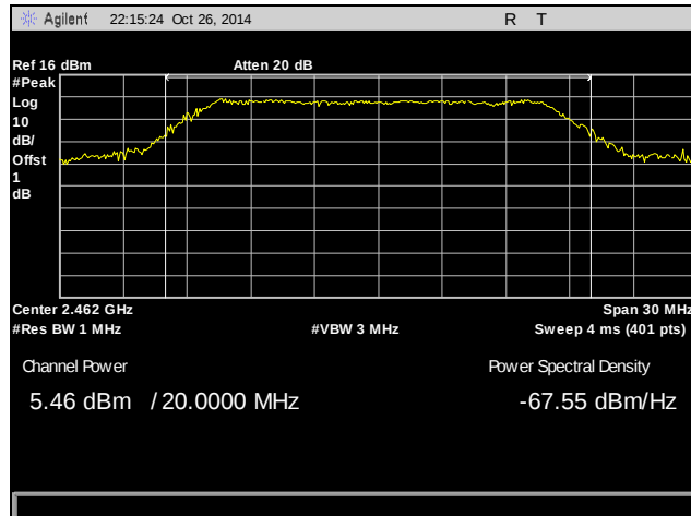
Plot 12. Peak Power Output, High Channel, 2462 MHz, 802.11g
