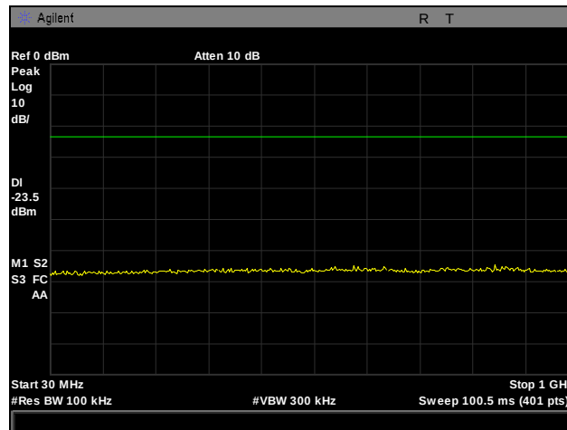
Plot 55. Conducted Spurious Emissions, High Channel, 2462 MHz, 802.11g, 30 MHz – 1 GHz
