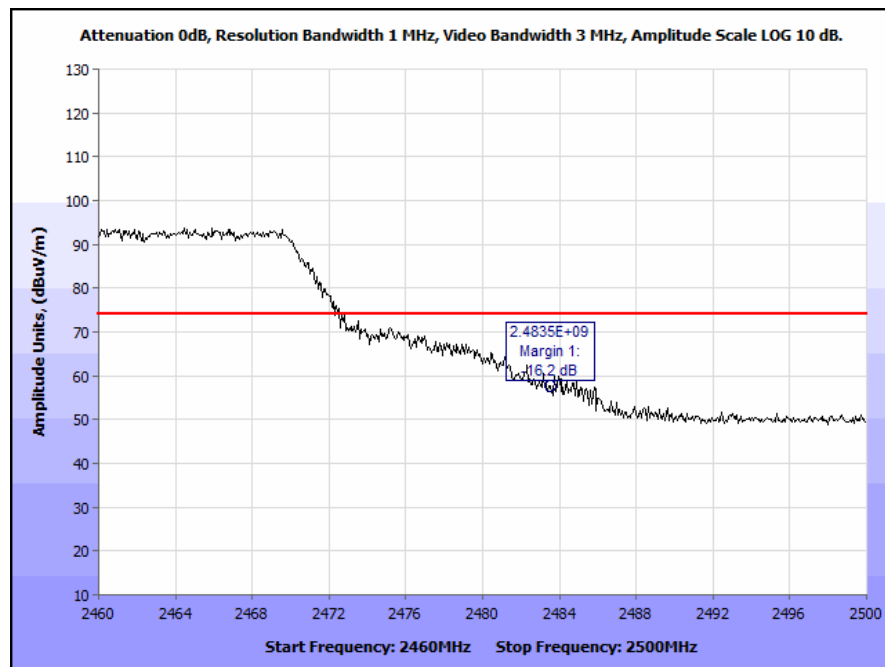
Plot 44. Radiated Band Edge, 802.11g, Channel 11, Peak
