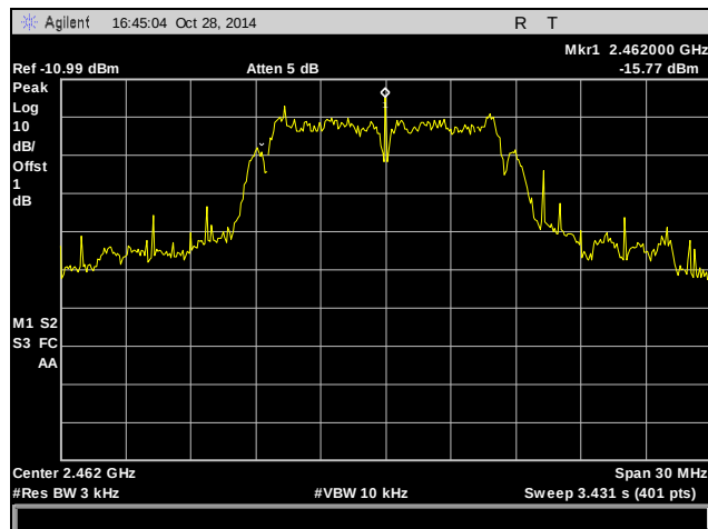
Plot 63. Peak Power Spectral Density, High Channel, 2462 MHz, 802.11b
