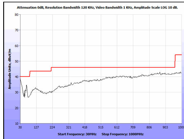
Plot 13. Radiated Spurious Emissions, Low Channel, 2412 MHz, 802.11g, 30 MHz – 1 GHz, Average
