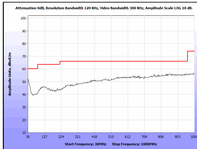
Plot 26. Radiated Spurious Emissions, Low Channel, 2412 MHz, 802.11n, 30 MHz – 1 GHz, Peak
