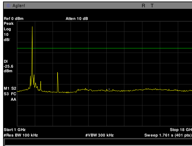
Plot 48. Conducted Spurious Emissions, Mid Channel, 2442 MHz, 802.11g, 1 GHz – 18 GHz
