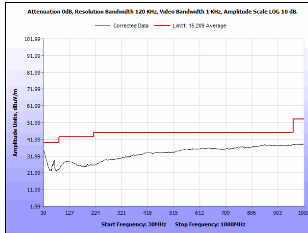
Plot 25. Radiated Spurious Emissions, Low Channel, 2412 MHz, 802.11n, 30 MHz – 1 GHz, Average
