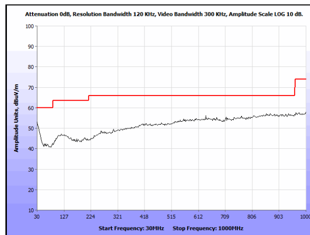
Plot 14. Radiated Spurious Emissions, Low Channel, 2412 MHz, 802.11g, 30 MHz – 1 GHz, Peak
