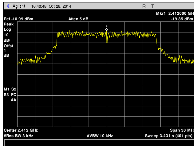
Plot 28. Peak Power Spectral Density, Low Channel, 802.11g
