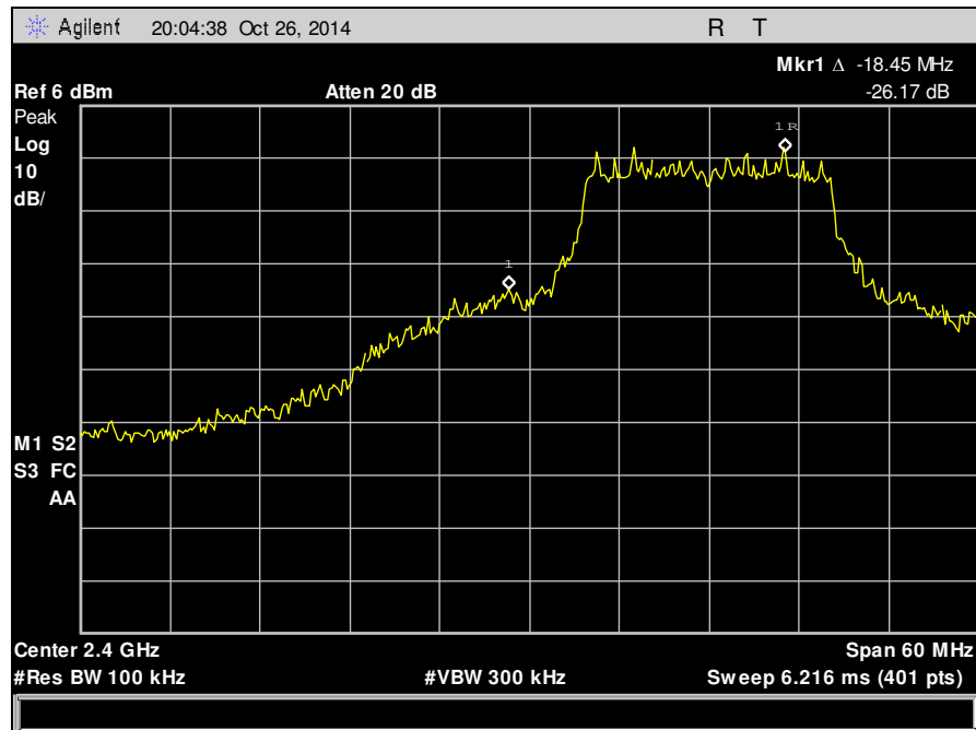
Plot 26. Conducted Band Edge, Low Channel, 802.11g
