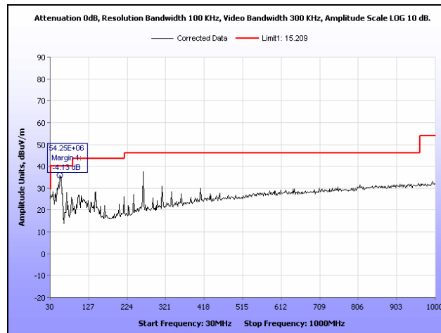
Plot 7. Radiated Spurious Emissions, Low Channel, 802.11g, 30 MHz – 1 GHz, Peak
