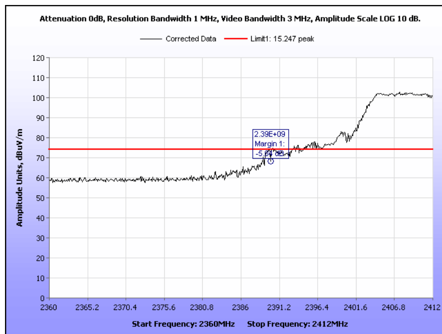
Plot 17. Radiated Restricted Band Edge, Low Channel, 802.11g, Peak
