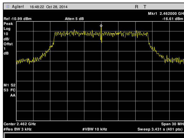
Plot 30. Peak Power Spectral Density, High Channel, 802.11g
