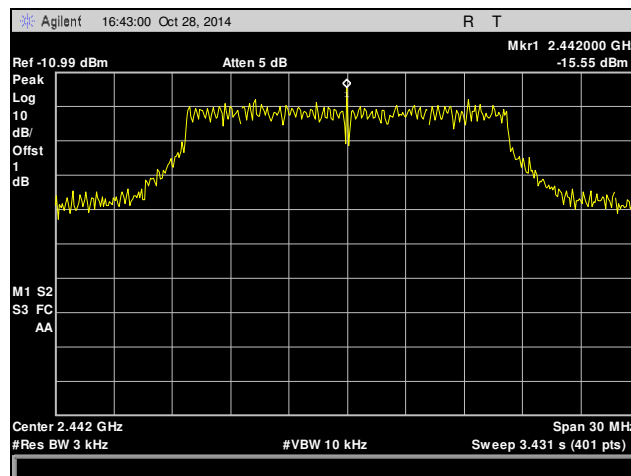
Plot 29. Peak Power Spectral Density, Mid Channel, 802.11g
