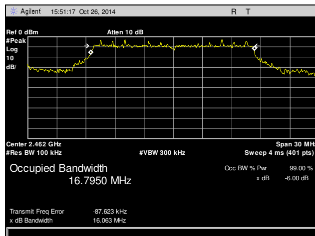
Plot 3. 6 dB Occupied Bandwidth, High Channel, 802.11g
