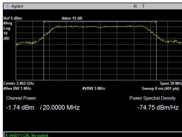
Plot 6. Peak Power Output, High Channel, 802.11g
