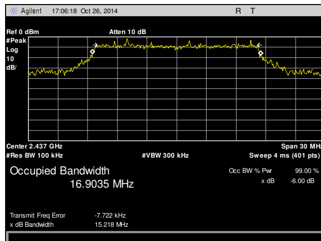
Plot 2. 6 dB Occupied Bandwidth, Mid Channel, 802.11g
