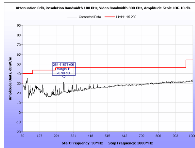
Plot 13. Radiated Spurious Emissions, High Channel, 802.11g, 30 MHz – 1 GHz, Peak
