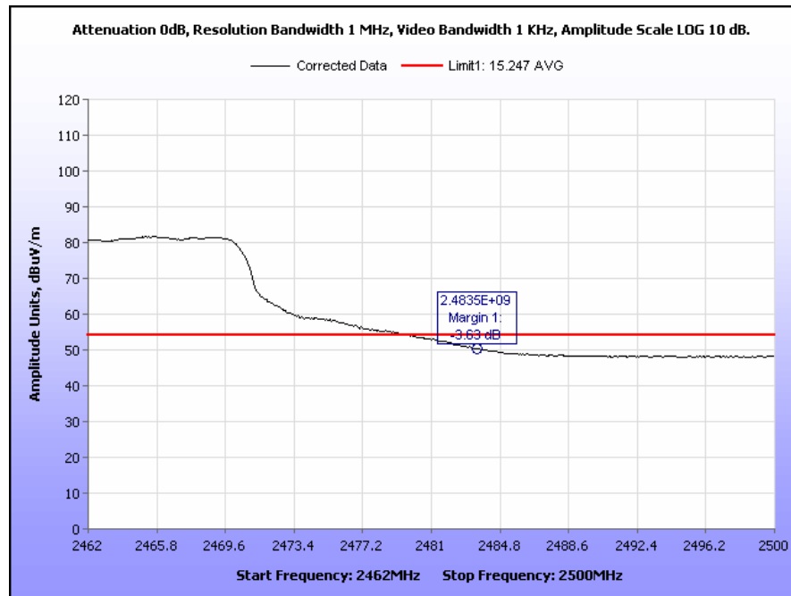
Plot 18. Radiated Restricted Band Edge, High Channel, 802.11g, Average
