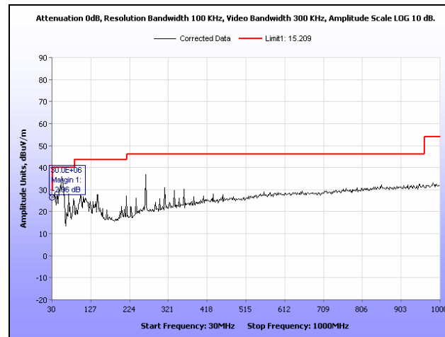
Plot 10. Radiated Spurious Emissions, Mid Channel, 802.11g, 30 MHz – 1 GHz, Peak
