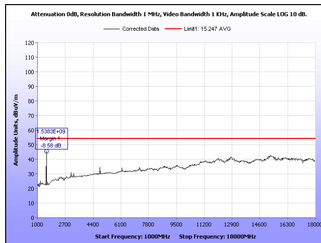
Plot 8. Radiated Spurious Emissions, Low Channel, 802.11g, 1 GHz – 18 GHz, Average
