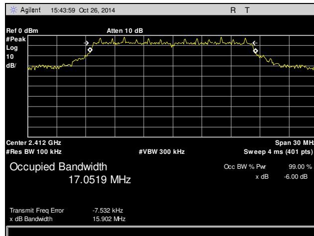
Plot 1. 6 dB Occupied Bandwidth, Low Channel, 802.11g
