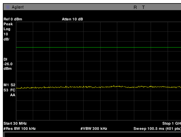
Plot 22. Conducted Spurious Emissions, Mid Channel, 802.11g, 30 MHz – 1 GHz
