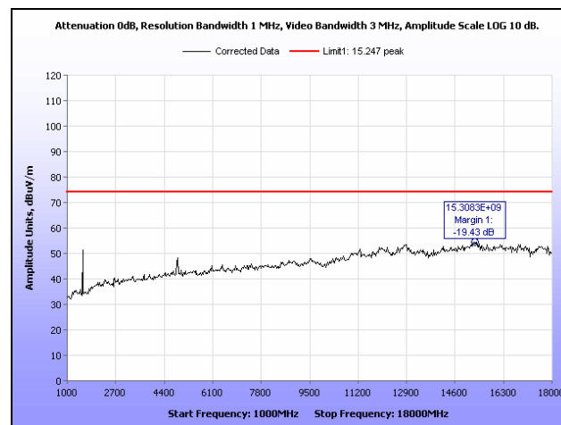
Plot 12. Radiated Spurious Emissions, Mid Channel, 802.11g, 1 GHz – 18 GHz, Peak
