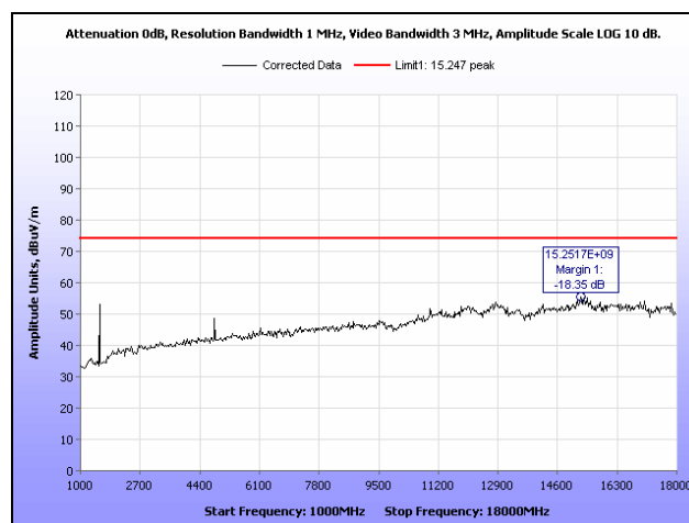
Plot 9. Radiated Spurious Emissions, Low Channel, 802.11g, 1 GHz – 18 GHz, Peak
