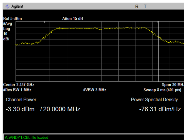
Plot 5. Peak Power Output, Mid Channel, 802.11g
