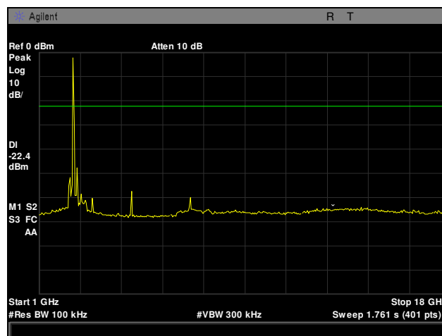
Plot 21. Conducted Spurious Emissions, Low Channel, 802.11g, 1 GHz – 18 GHz
