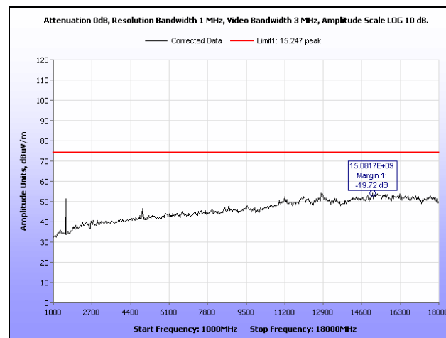
Plot 15. Radiated Spurious Emissions, High Channel, 802.11g, 1 GHz – 18 GHz, Peak
