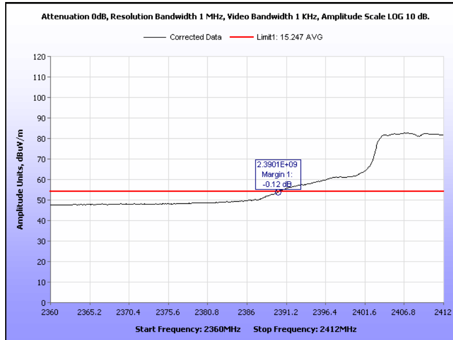
Plot 16. Radiated Restricted Band Edge, Low Channel, 802.11g, Average
