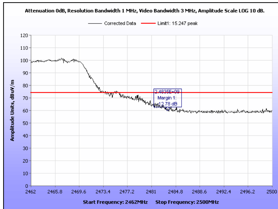
Plot 19. Radiated Restricted Band Edge, High Channel, 802.11g, Peak
