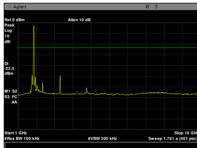
Plot 25. Conducted Spurious Emissions, High Channel, 802.11g, 1 GHz – 18 GHz
