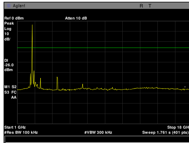
Plot 23. Conducted Spurious Emissions, Mid Channel, 802.11g, 1 GHz – 18 GHz
