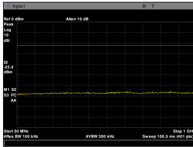
Plot 20. Conducted Spurious Emissions, Low Channel, 802.11g, 30 MHz – 1 GHz
