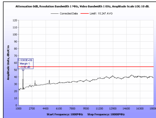
Plot 11. Radiated Spurious Emissions, Mid Channel, 802.11g, 1 GHz – 18 GHz, Average
