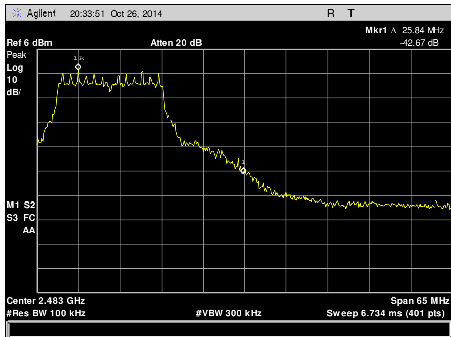
Plot 27. Conducted Band Edge, High Channel, 802.11g
