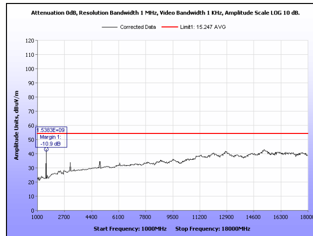
Plot 14. Radiated Spurious Emissions, High Channel, 802.11g, 1 GHz – 18 GHz, Average
