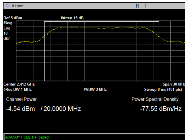
Plot 4. Peak Power Output, Low Channel, 802.11g
