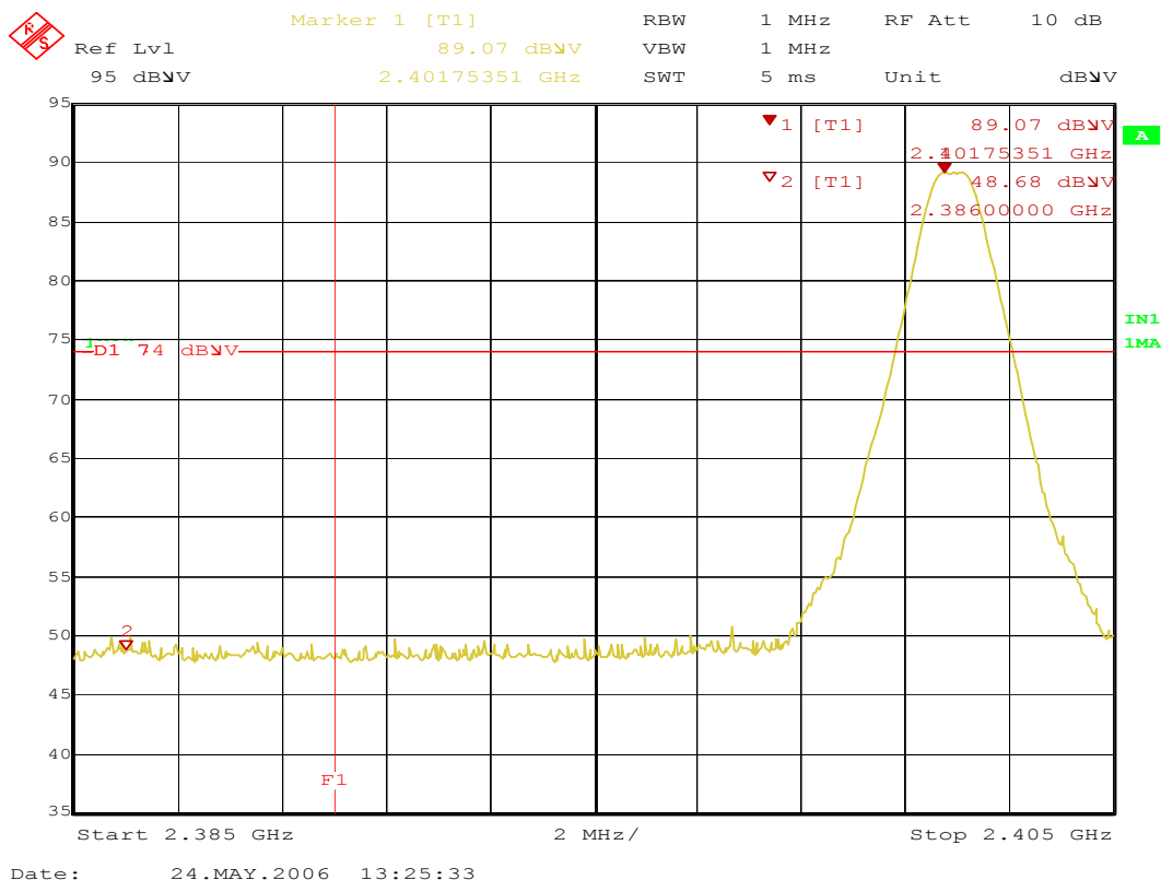
Figure 7. Plot of the Band Edge (Radiated)
