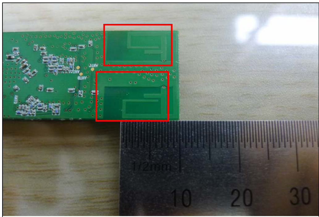
WLAN Module – Internal PCB Antenna
