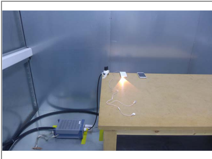
Photo of Conducted power line test
