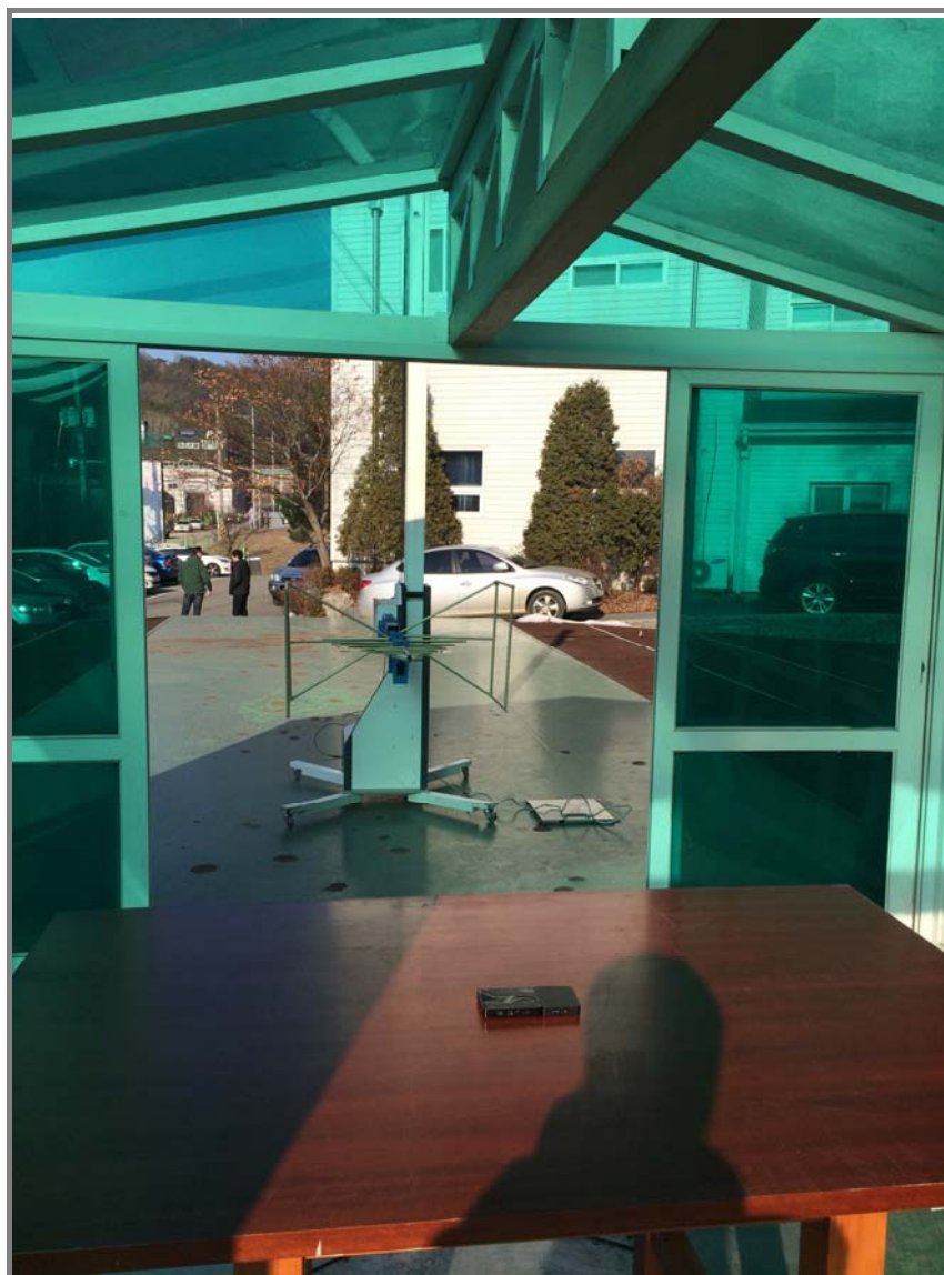
Photo of radiated spurious emission at 30 MHz ~ 1 000 MHz
