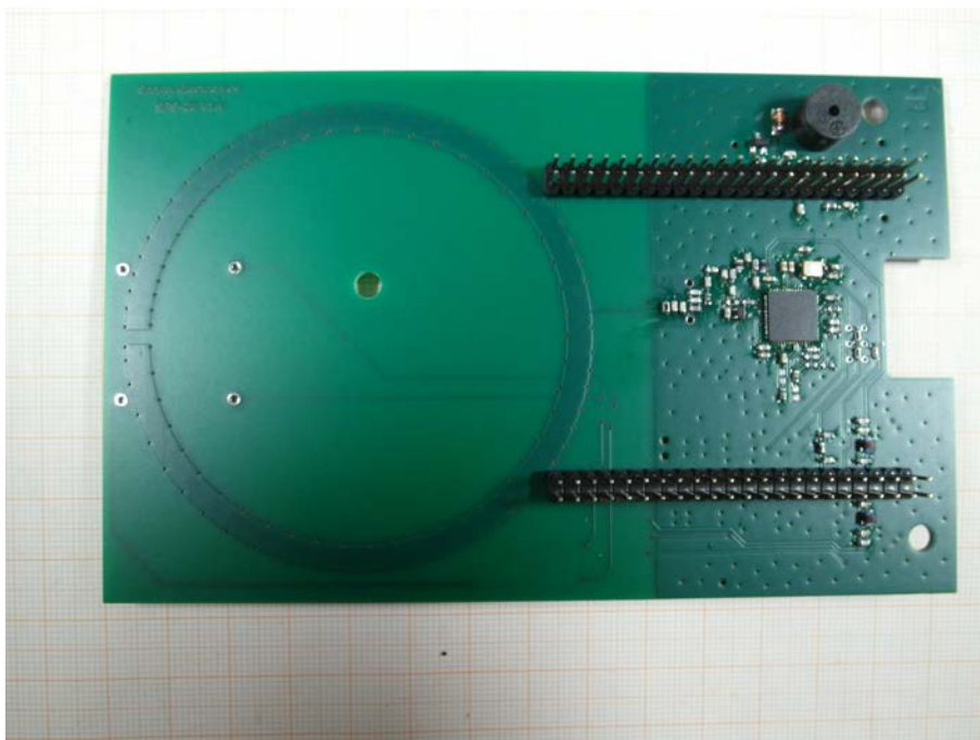
Photo 2: RF – Board connection side
