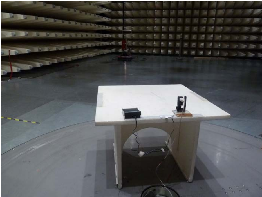
Photo 5: Test setup for radiated above 30 MHz
