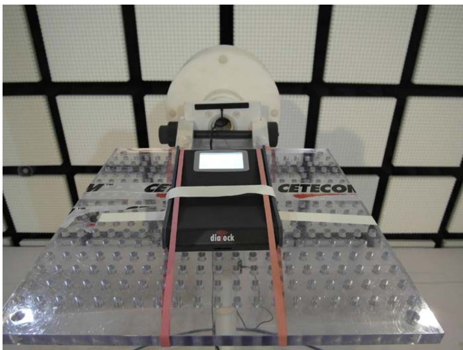
Photo 4: Test setup for radiated 9 kHz to 30 MHz
