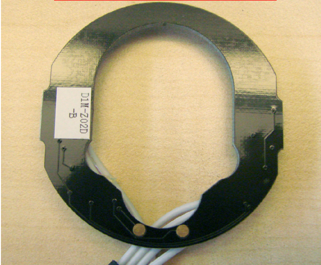
DT700-BLE / DT710-BLE RFID antenna pcb (SHS-92) bottom view
