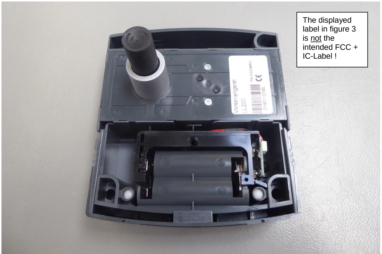
Figure 3 - Rear View 2
