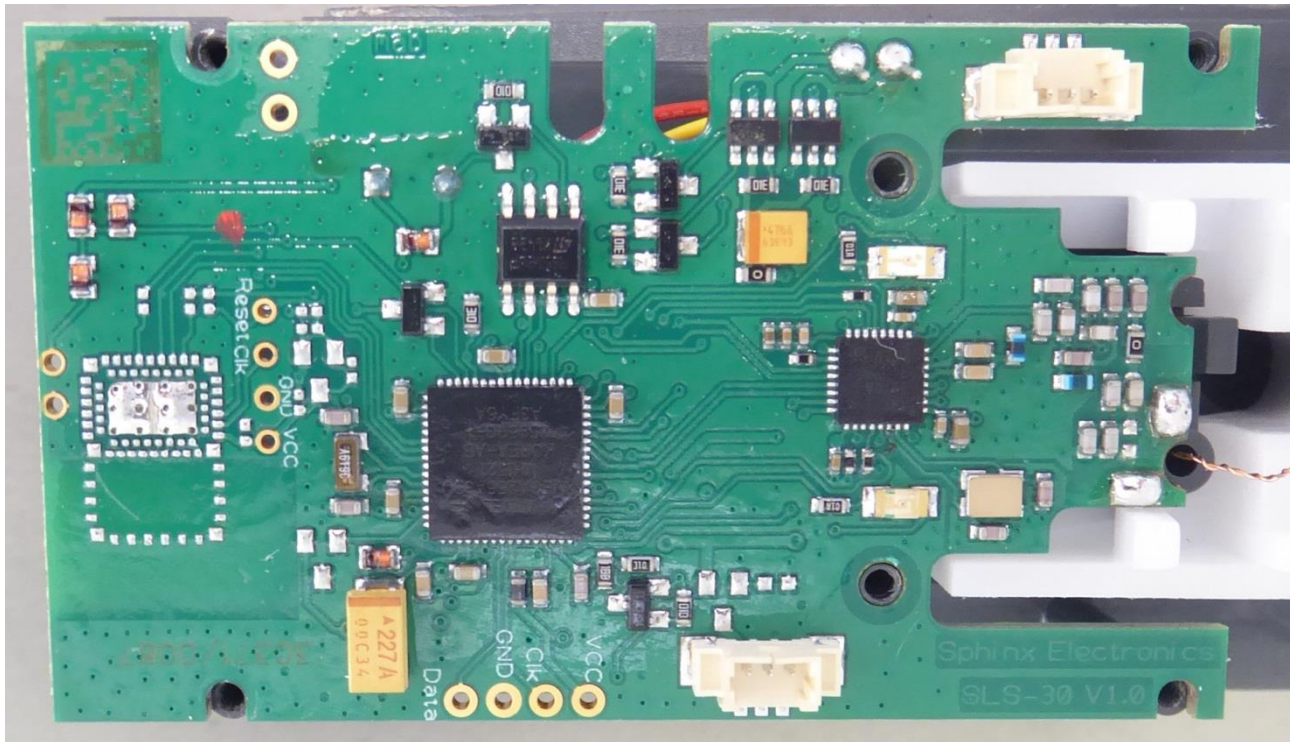
Figure 9 - SHS-30 v1.0 Top View
