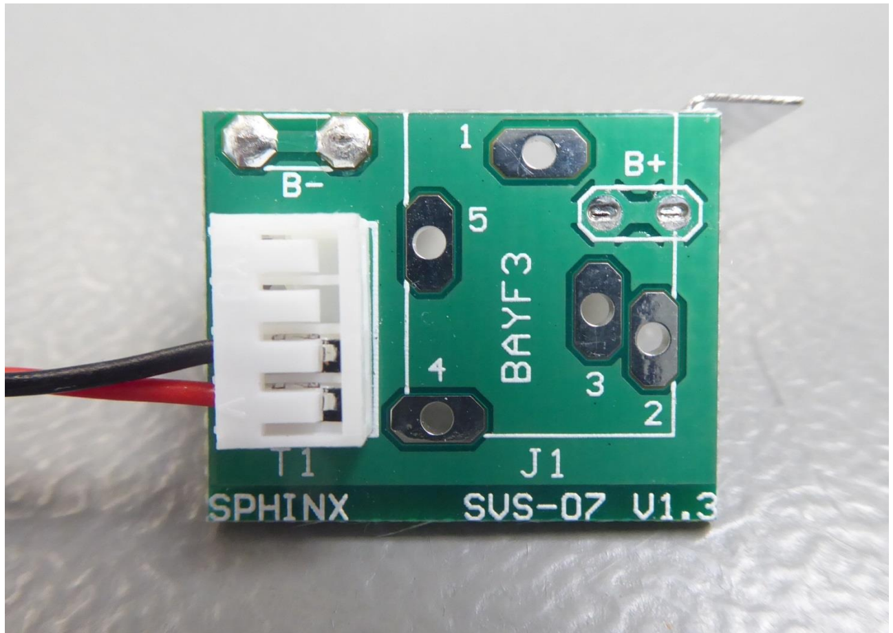
Figure 11 - SVS-07 v1.3 Top View
