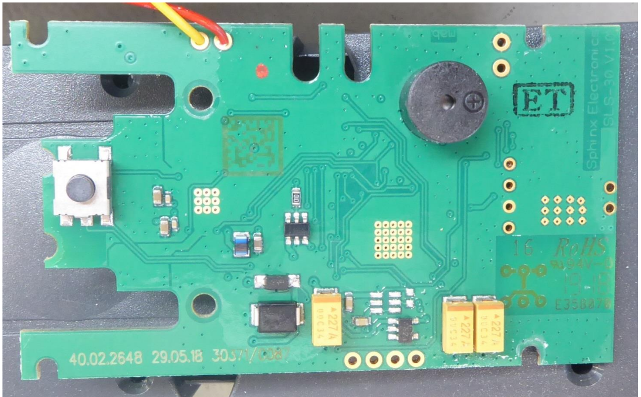
Figure 10 - SHS-30 v1.0 Bottom View
