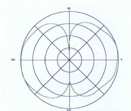
Vertical radiation diagram
