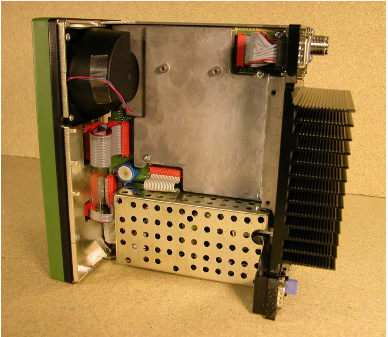
Cover removed to Base band with rf screen. Keyboard/display at left. Loudspeaker at upper left corner. Power supply module in metal box at bottom
