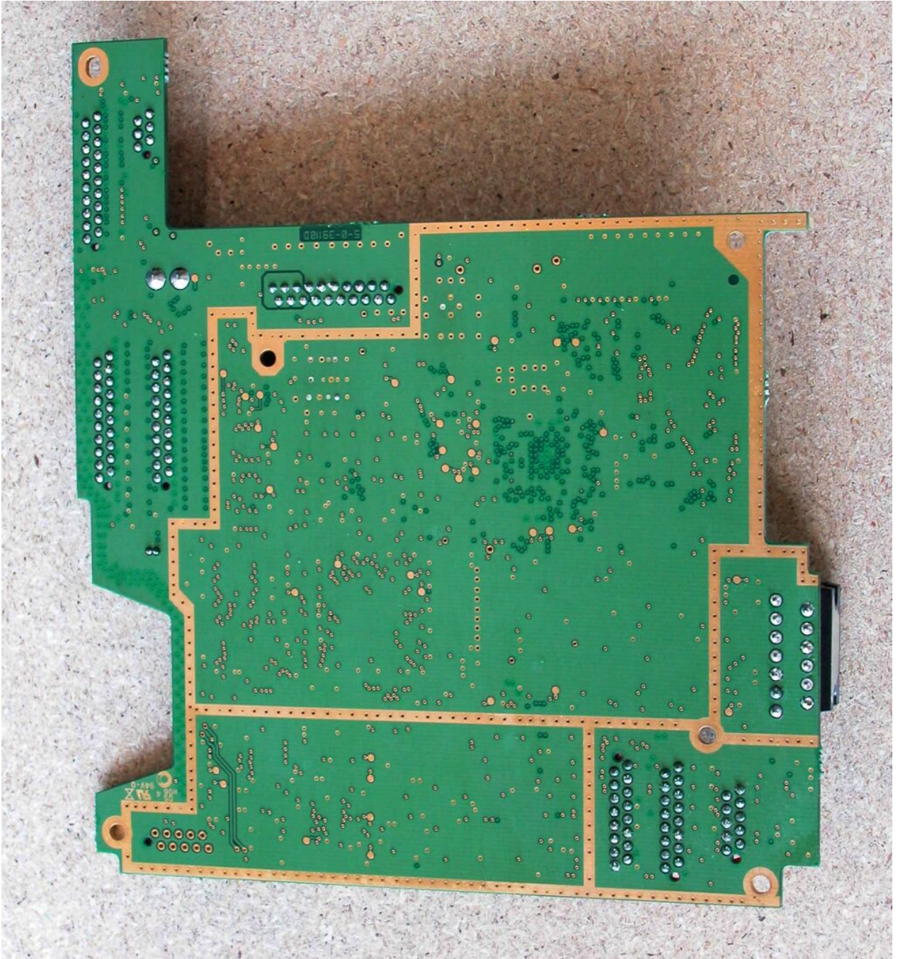
Base Band module 639110, lower layer
