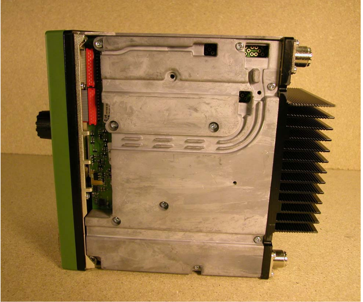
Cover removed to Rf module with Rf screen
