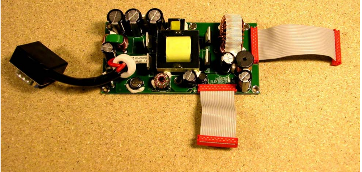
Power supply module, upper layer
