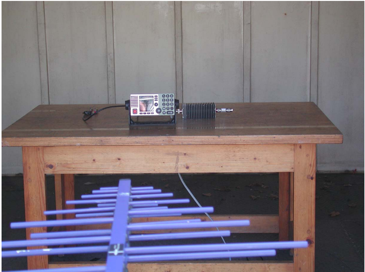
Photograph 1: Radiated emissions test set-up (OATS)
