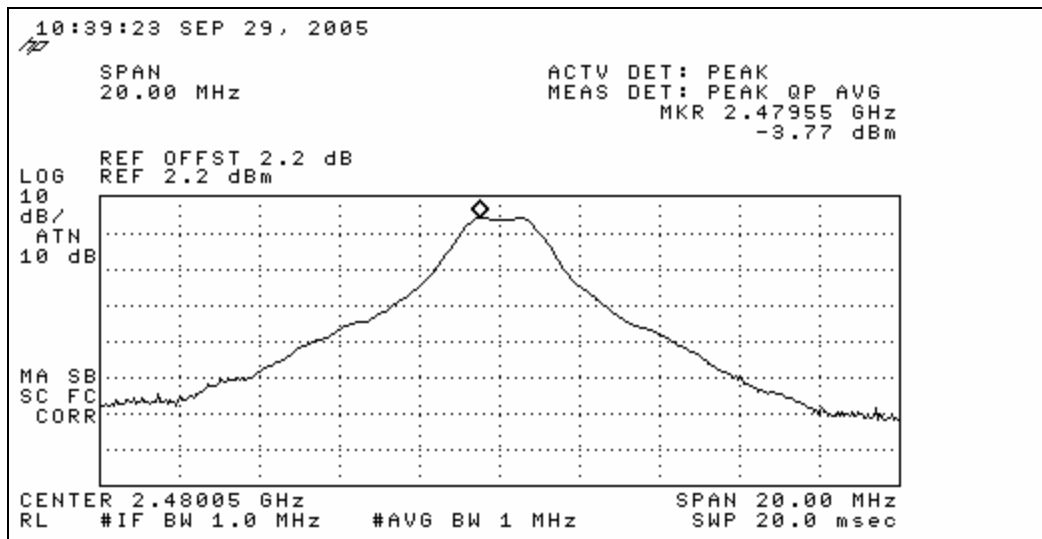
Plot 6 High Channel (2480 MHz) Power
