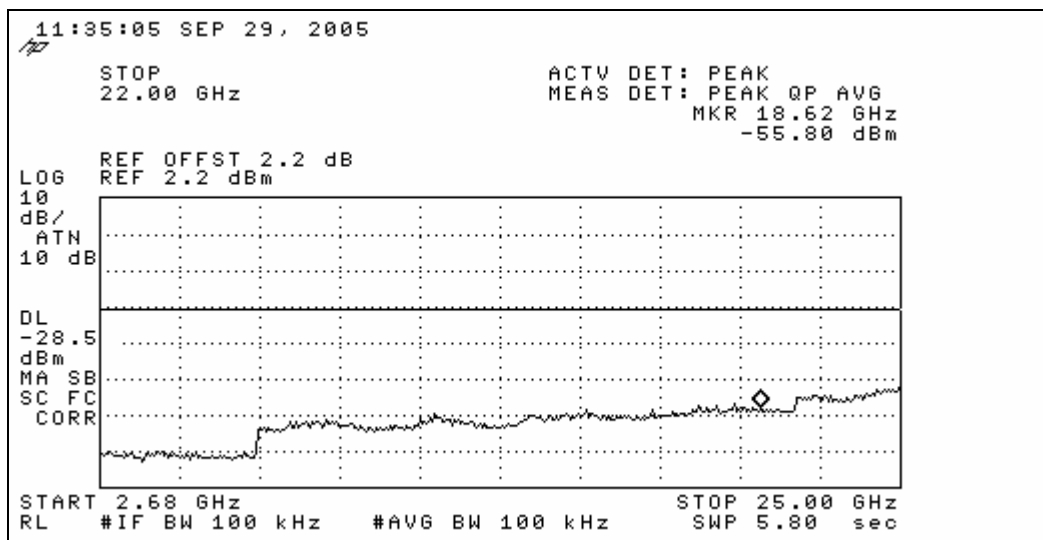
Plot 12 Mid-channel (2441 MHz) Spurious Emission, 2.68 GHz - 25 GHz
