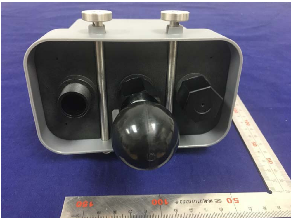
(4) EUT Photo (Flex AP ED)
