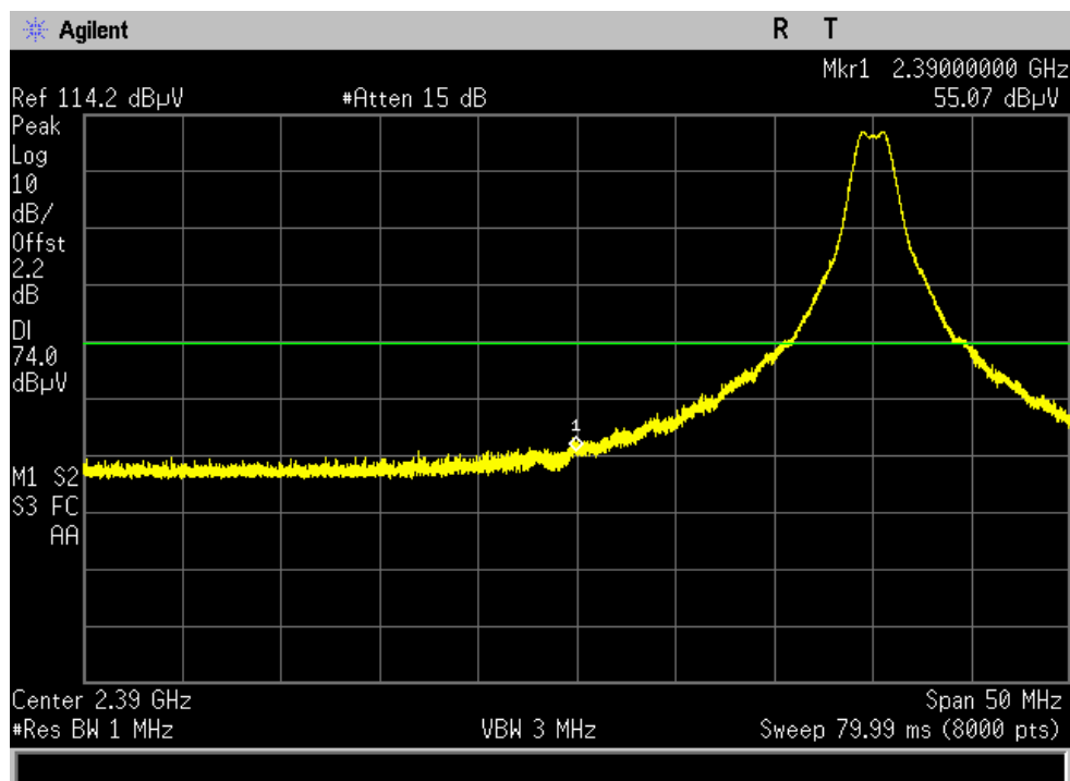
Band Edge- Low Channel- 15.209 - 14 dBi - Peak
