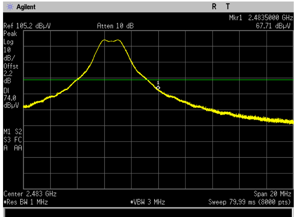
Band Edge- High Channel- 15.209 - 14 dBi - Peak
