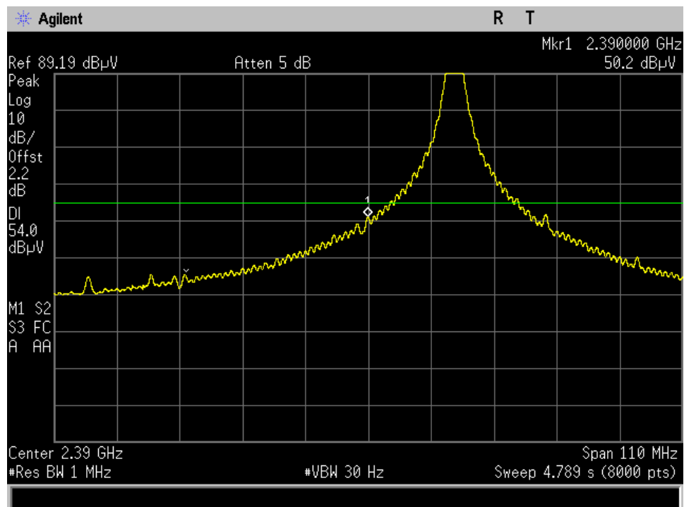
Band Edge- Low Channel- 15.209 - 14 dBi - Average
