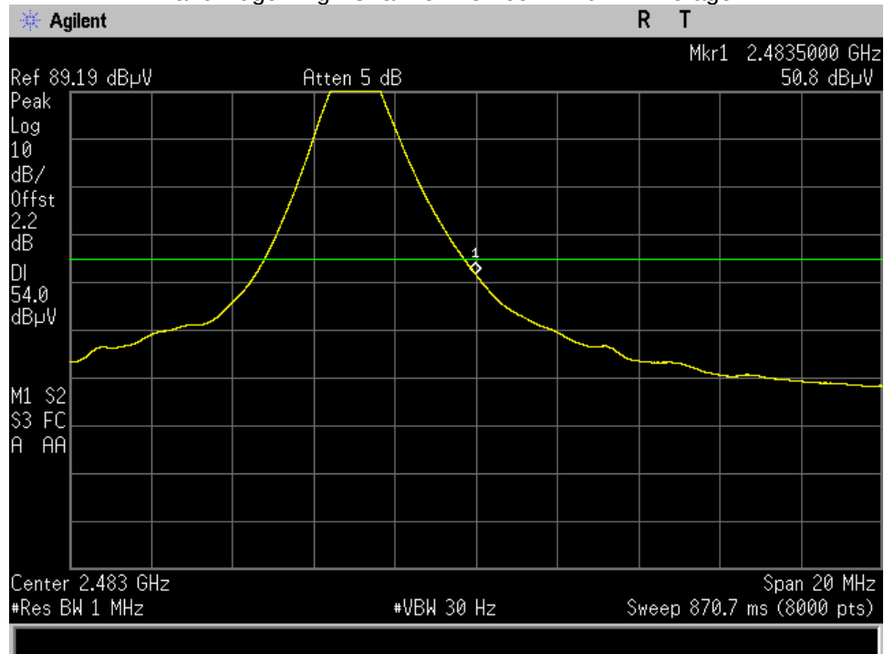
Band Edge- High Channel- 15.209 - 14 dBi - Average
