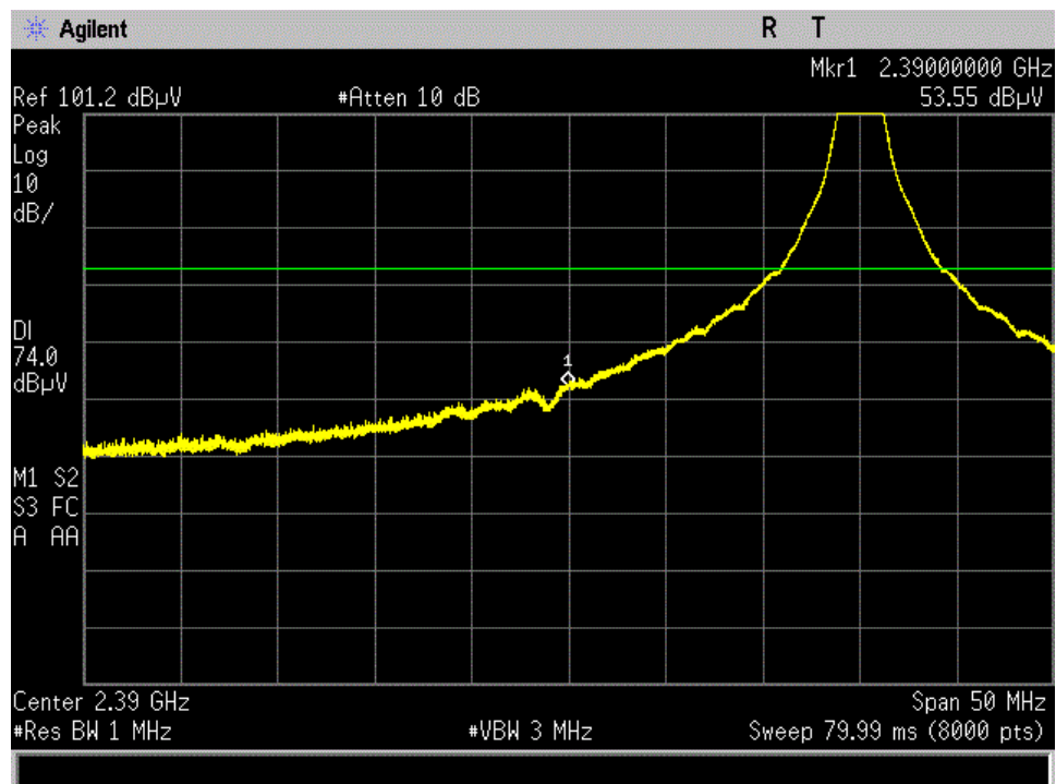
Band Edge- Low Channel- 15.209 - 5.5 dBi - Peak
