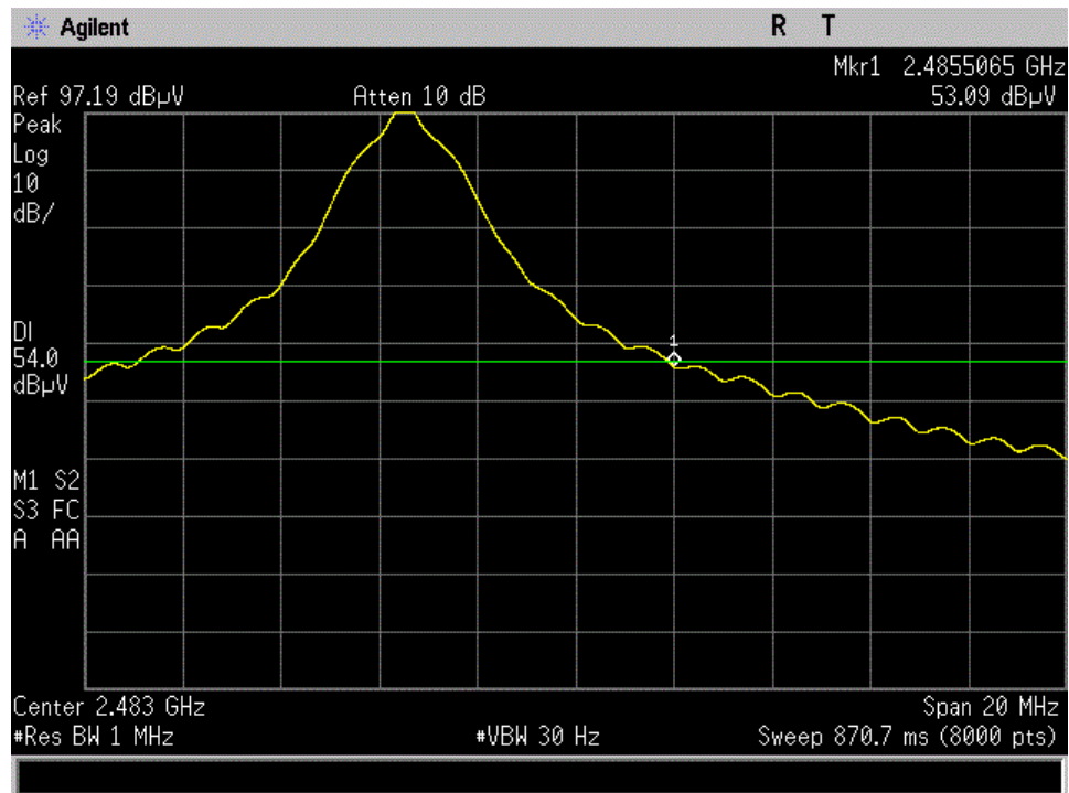
Band Edge- High Channel- 15.209 - 5.5 dBi - Peak
