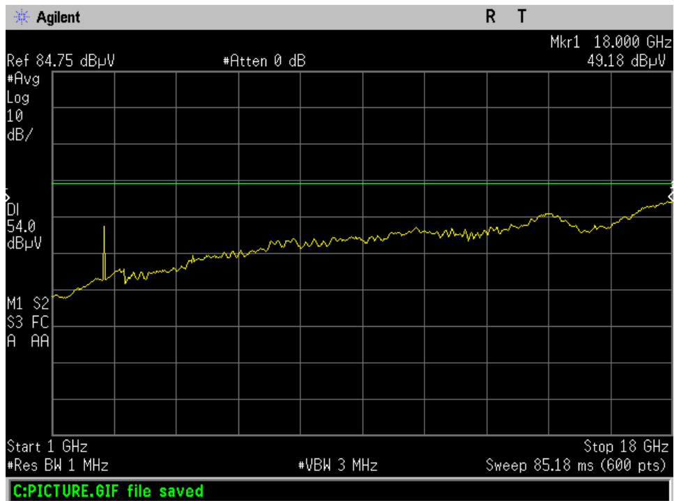
1-18 Ghz Mid Channel Peak- 5.5 dBi
