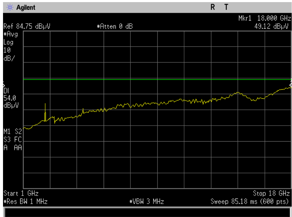
1-18 Ghz Low Channel Peak - 5.5 dBi
