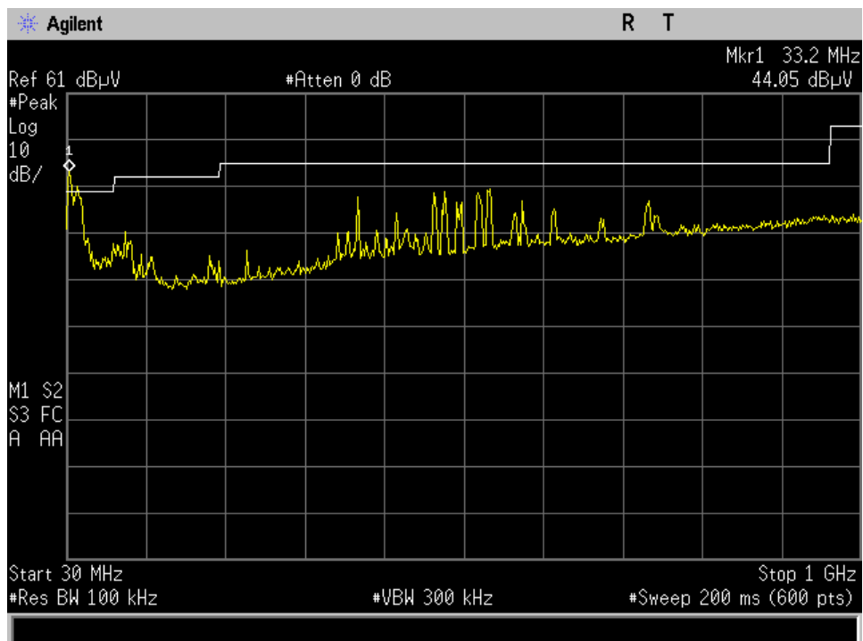
Standby Mode 30Mhz-1GHz
