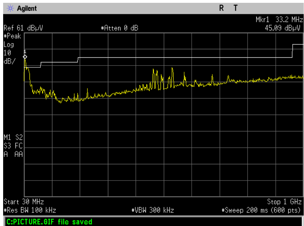
Low Channel- 30MHz- 1GHz- 209- 5.5 dBi
