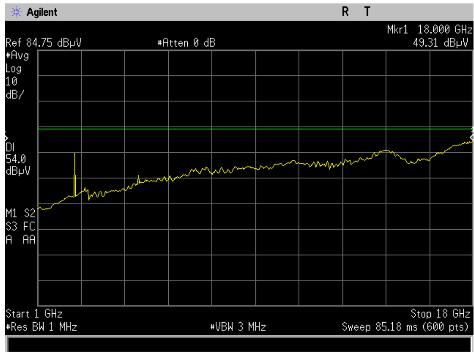
1-18 Ghz High Channel Peak- 5.5 dBi
