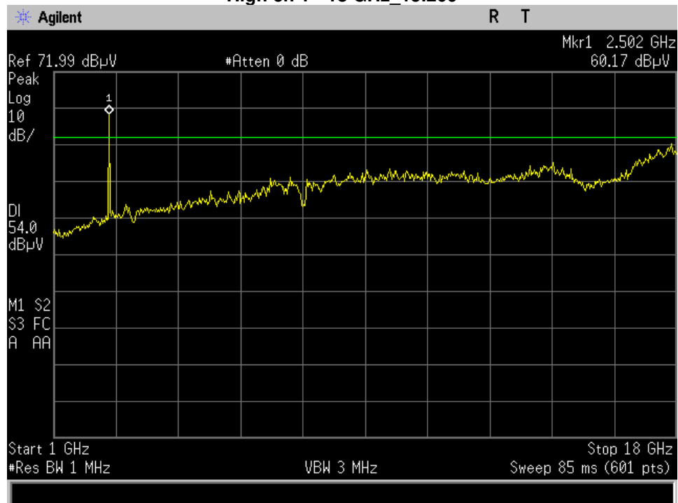
High ch 1 - 18 GHz_15.209
