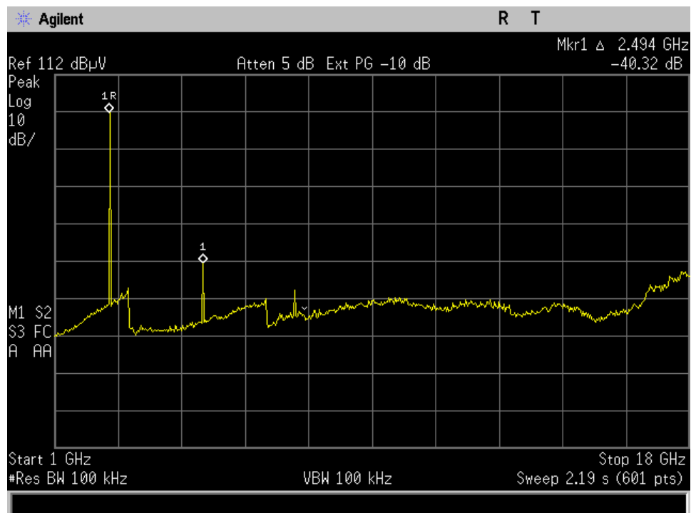
High ch 1 - 18 GHz_15.247
