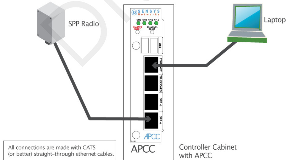
Figure 5.3. Cabling a PC or laptop
