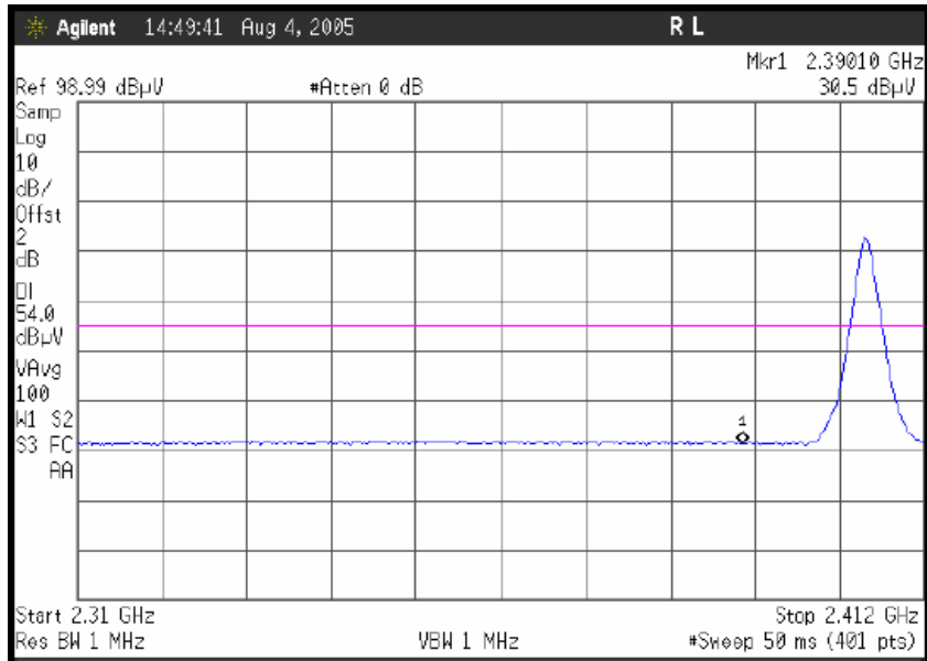
AVERAGE Limit at Vertical polarization, Lower Edge
