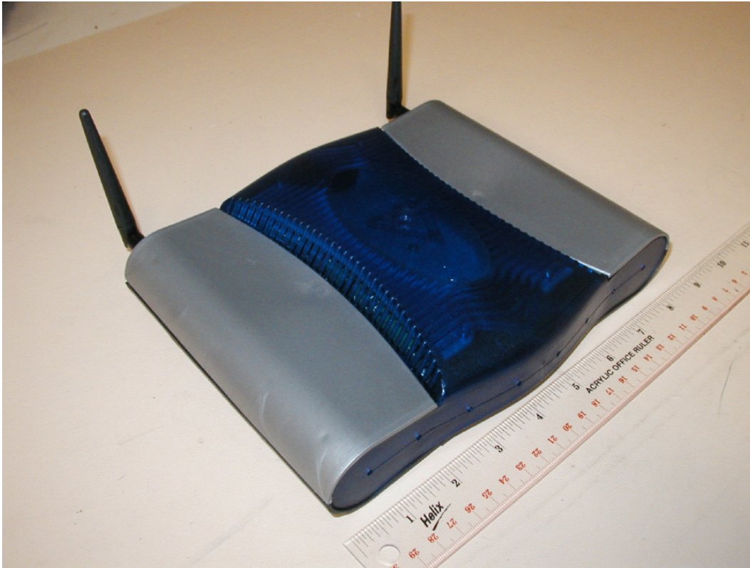
TDK-BWR54G1 external photos, June 16, 2005
