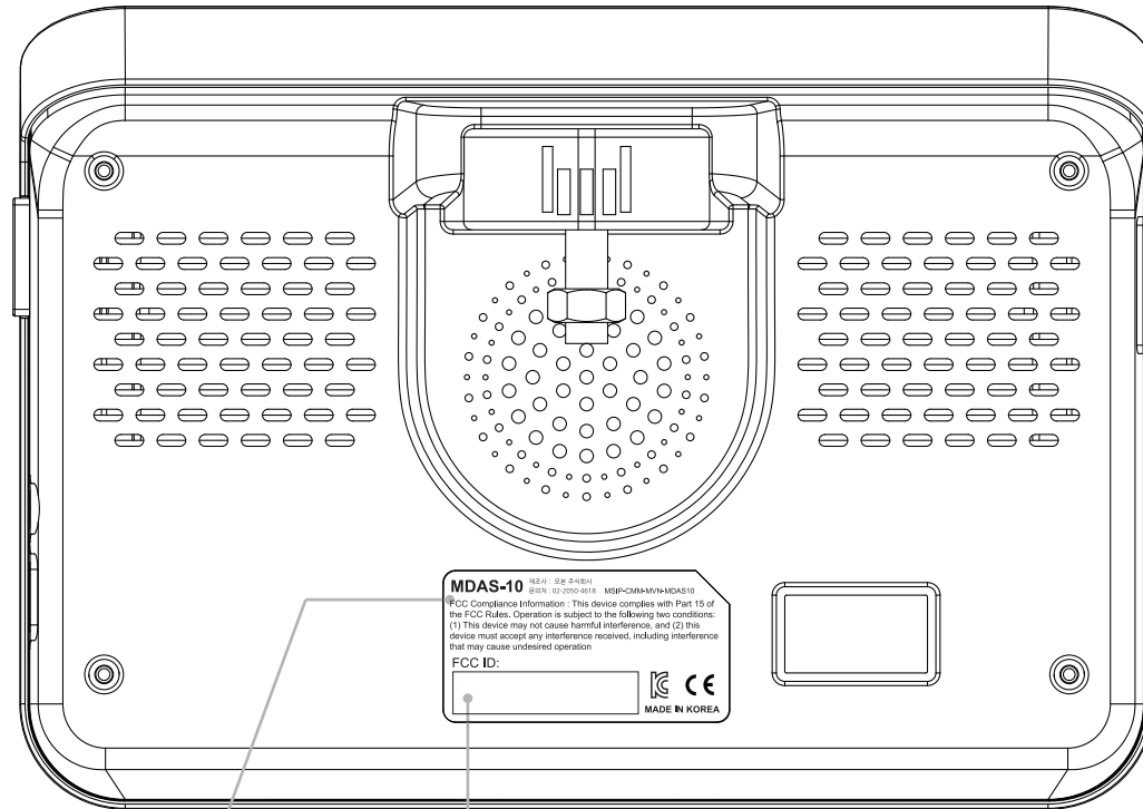
Bottom Cover
