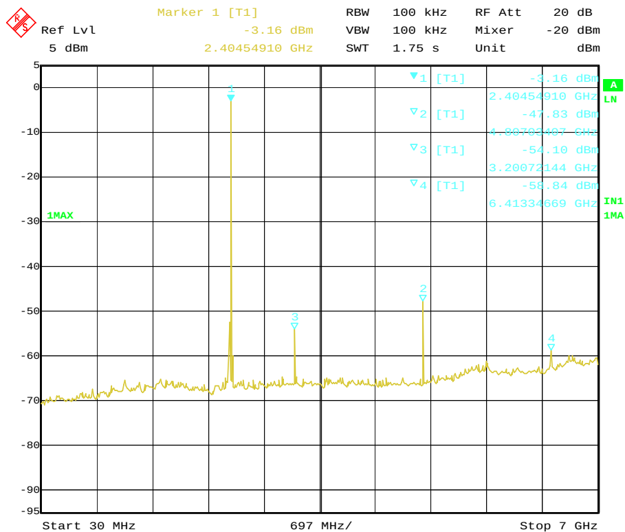
Figure 8. Plot of the RF antenna port emissions (Conducted)
