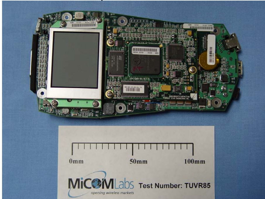
StarMOBILE Main Assy Top with LCD Assy p/n 810-00003-00
