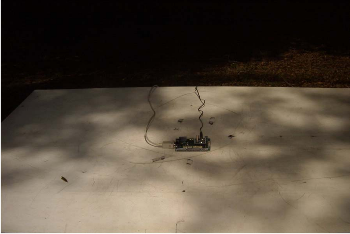
RADIATED EMISSIONS TEST SET UP WITH HELICAL ANTENNA, RFM PART NO. 500-1141-001
