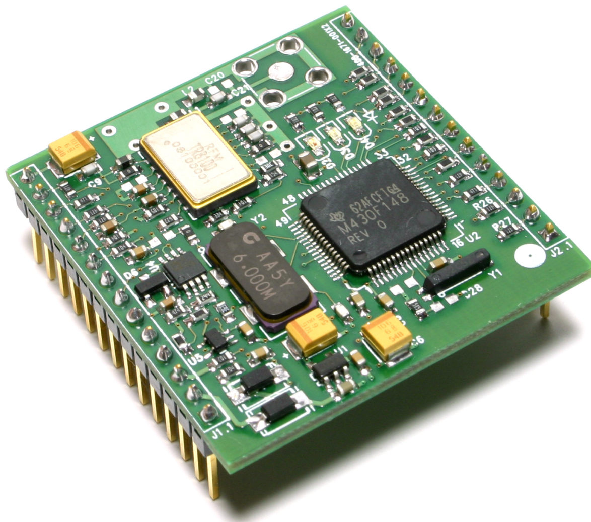
DM2200 Module FCC Reference Photo #1
