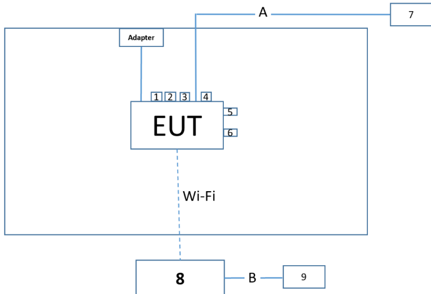
Connection Diagram- Radiated Emission testing (Beam-Forming mode)
