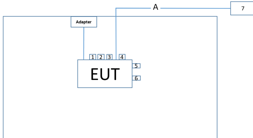
Connection Diagram- Radiated Emission testing (Beam-Forming mode)
