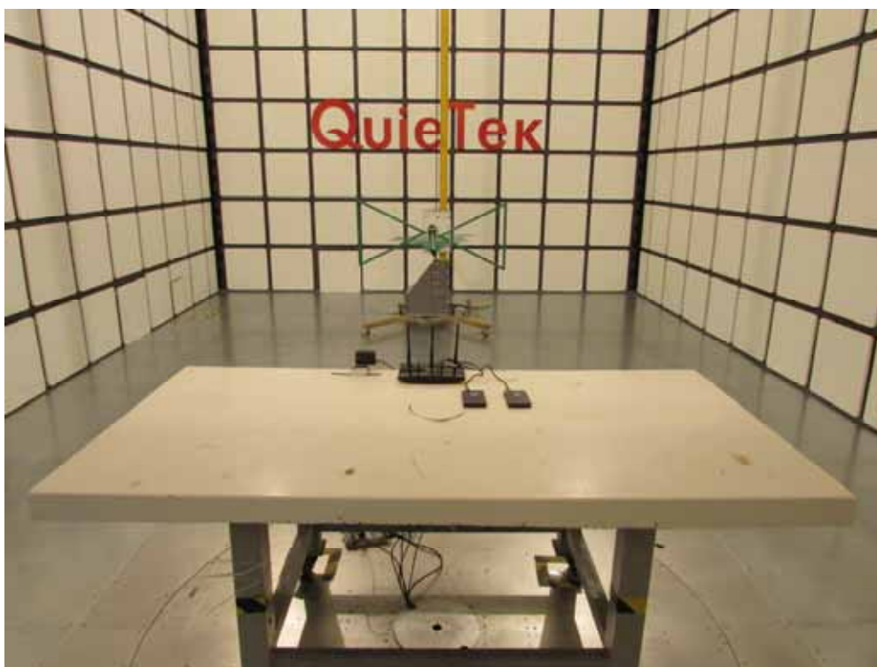
Description: Radiated Emission Test Setup for Below 1GHz
