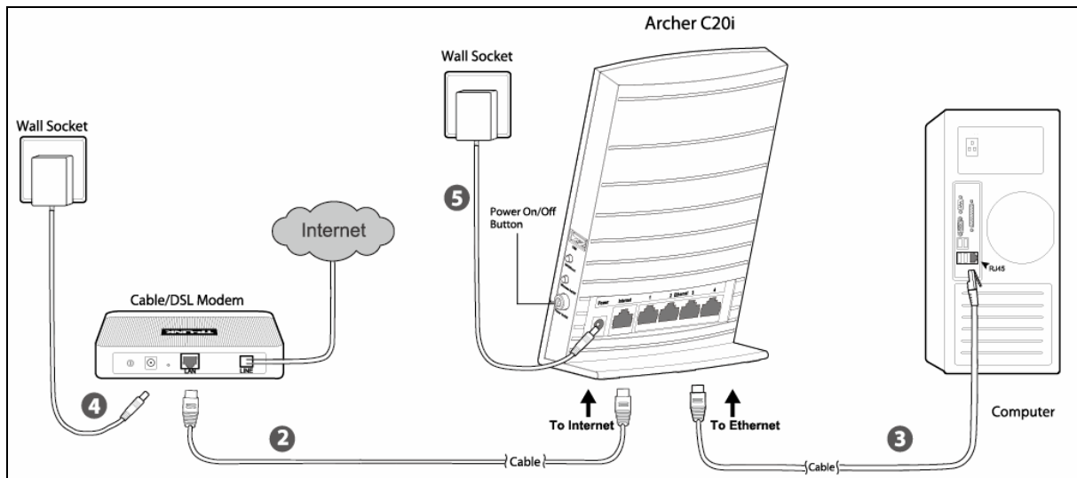
Figure 2-1 Hardware Installation
