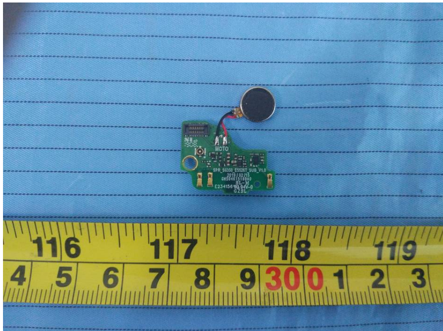
EUT – Connection PCB Top View
