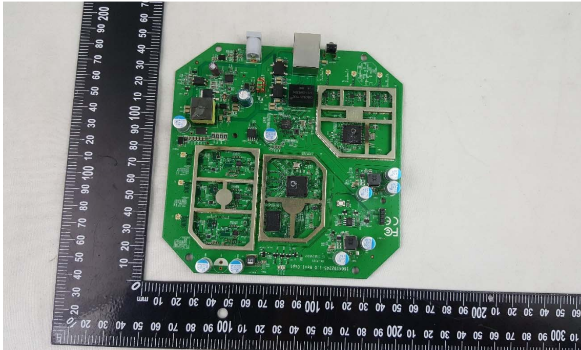
MAIN BOARD TOP VIEW 1
